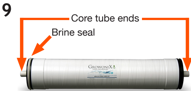
Pull the old membrane element out towards the input side of the membrane housing.
