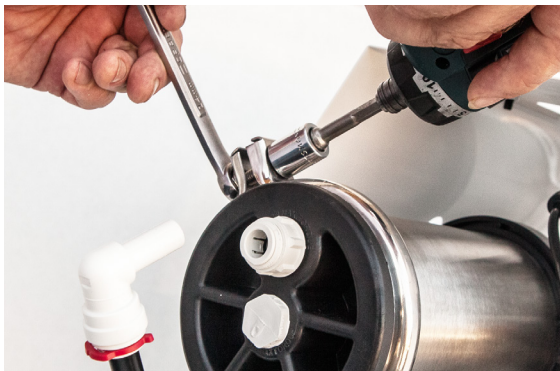
Tighten the stainless clamp retaining bolts evenly.
