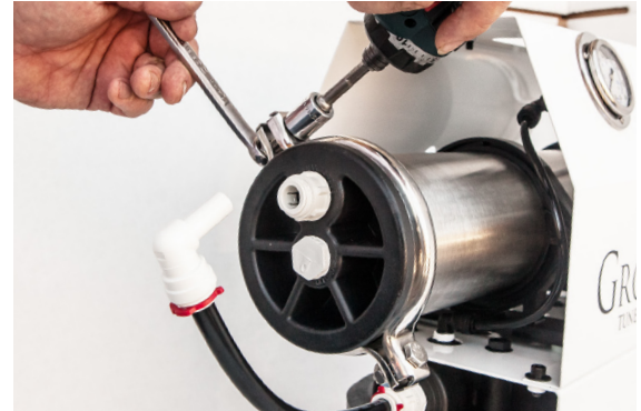
Replace the stainless clamp on the input side of the membrane housing.
