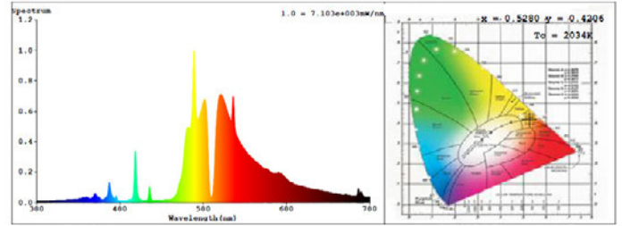
1000W spectral distribution
