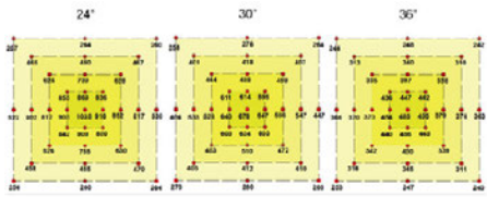
Light spread diagram
