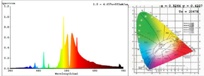
600W spectral distribution
