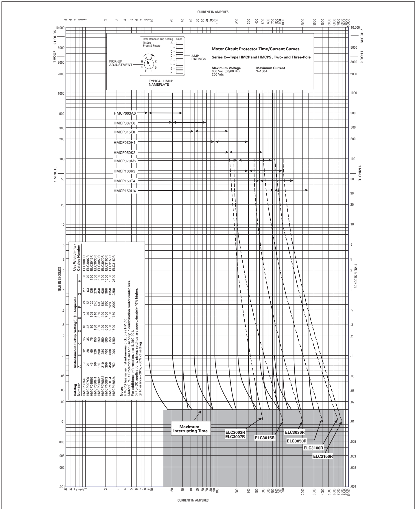
Figure 2. Type HMCP and HMCPs 150A Motor Circuit Protector—Curve No. SC-4121-87B
