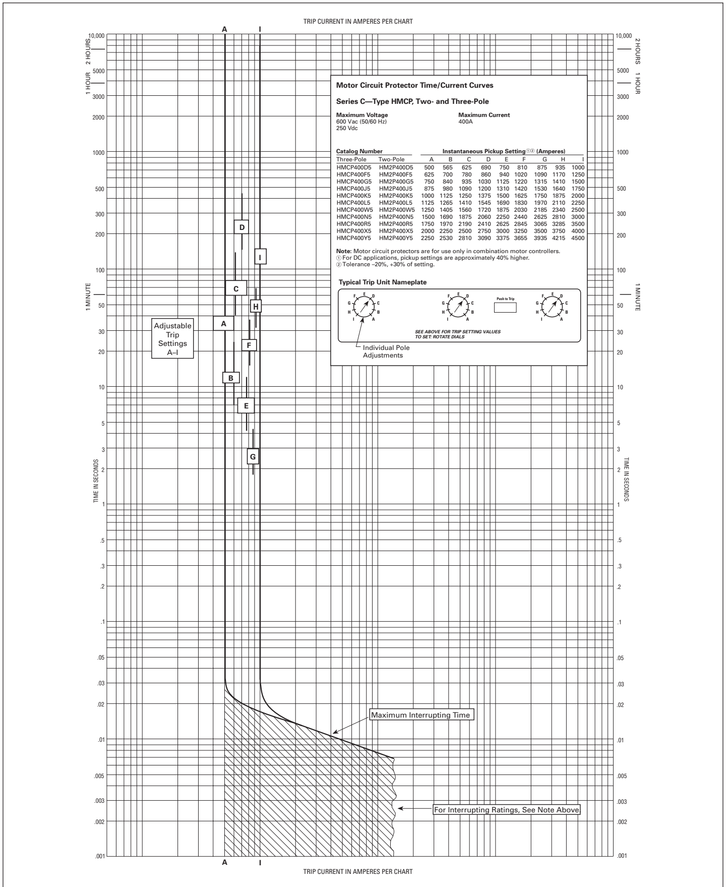
Figure 4. Type HMCP 400A Motor Circuit Protector—Curve No. SC-4420-88B
