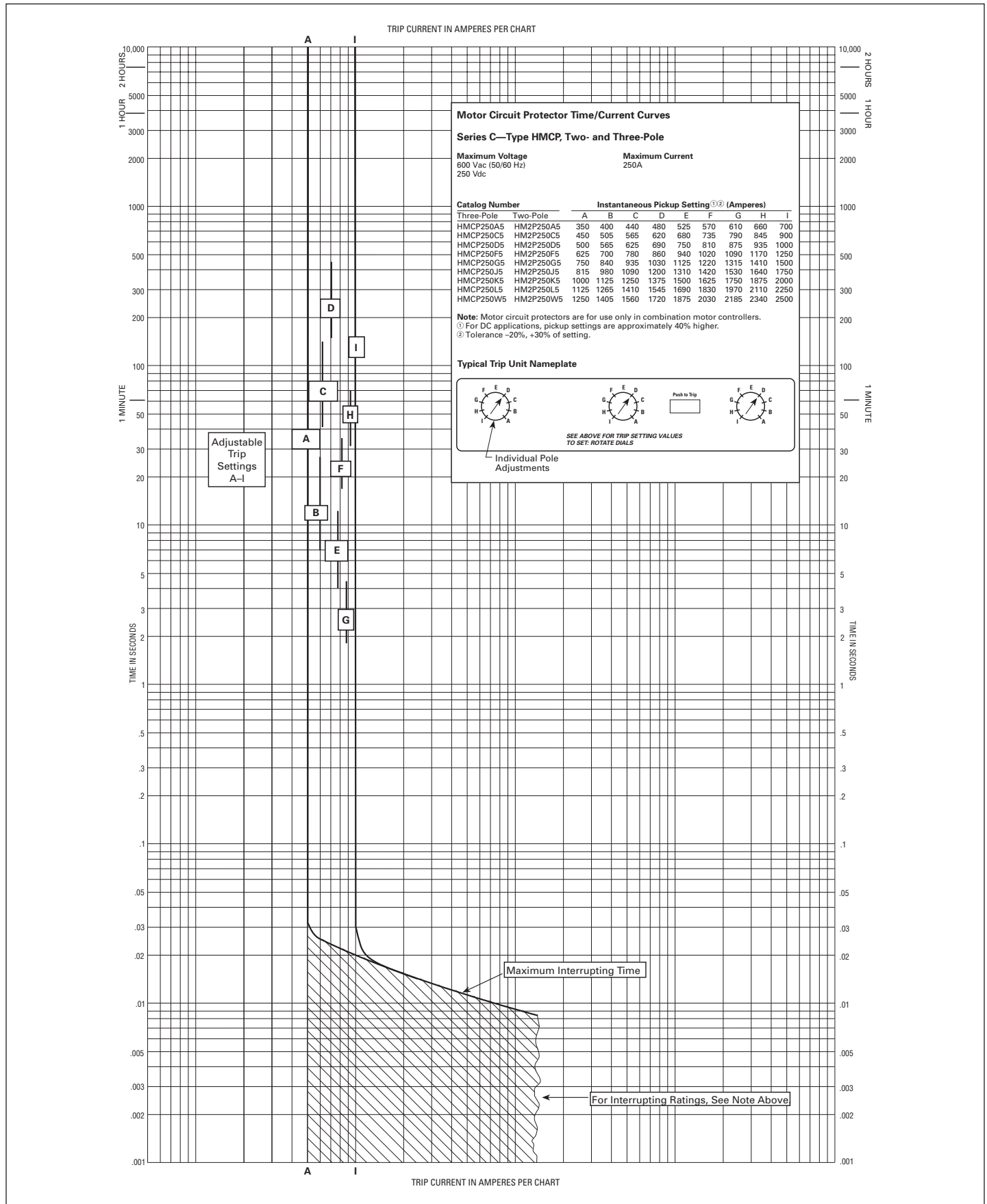
Figure 3. Type HMCP 250A Motor Circuit Protector—Curve No. SC-4419-88B
