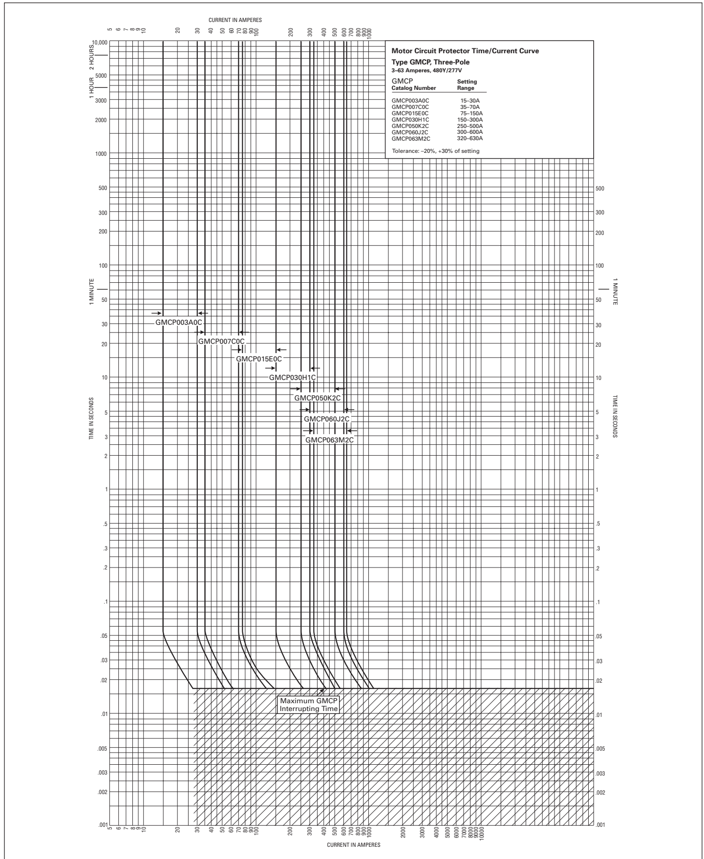
Figure 1. Type GMCP 63A Motor Circuit Protector—Curve No. SC-5670-93A
