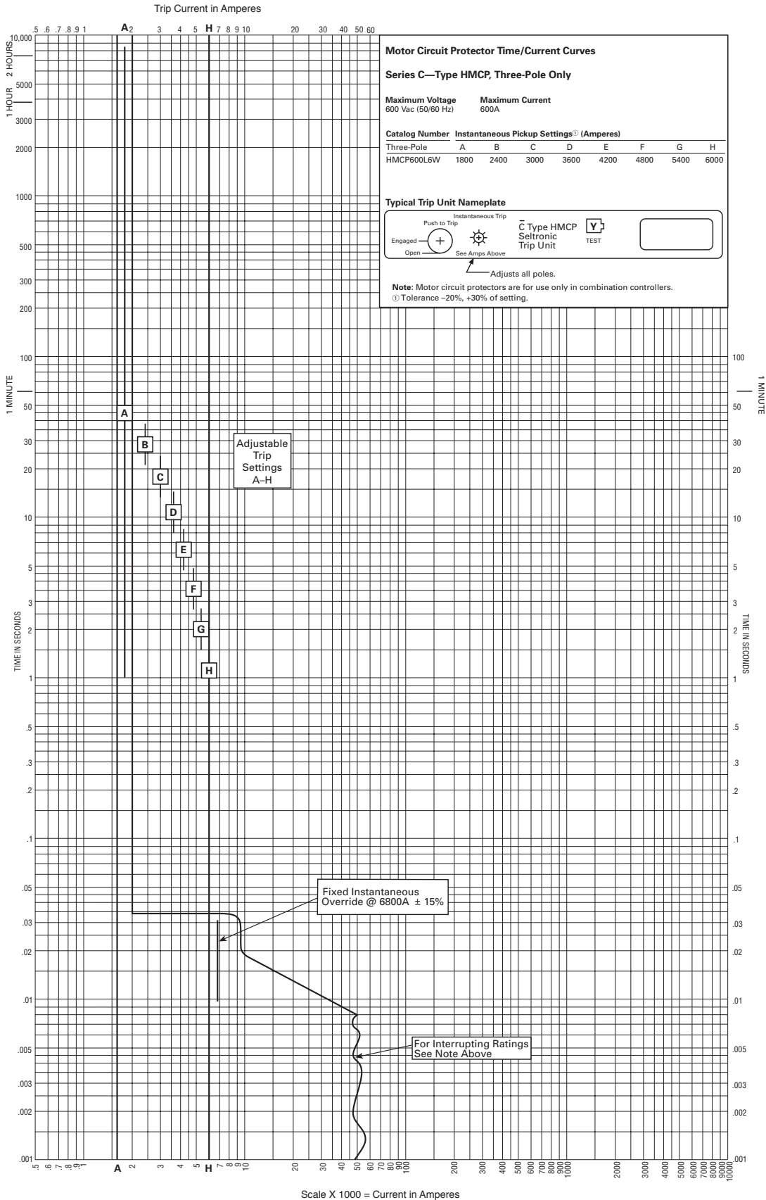
Figure 5. Type HMCP 600A Motor Circuit Protector—Curve No. SC-5373-93A
