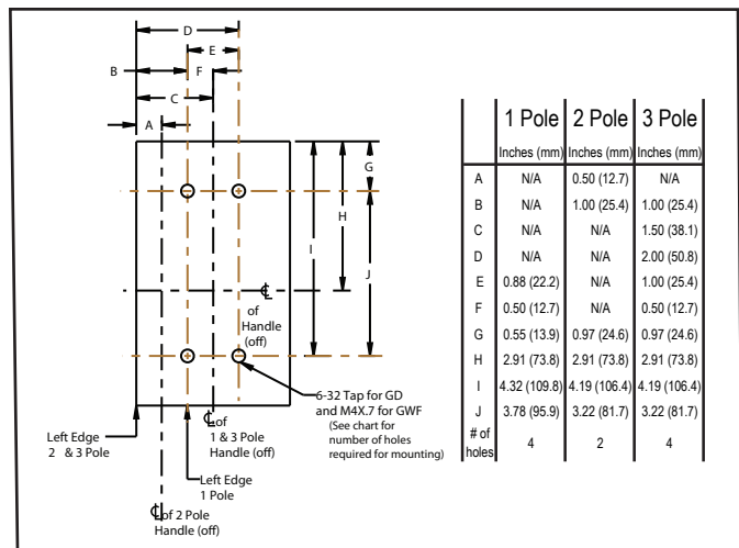
Figure 2-1 Circuit Breaker Mounting Bolt Drilling Plan
