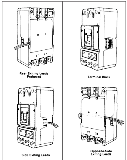
Fig. 2-2. Accessory Wiring Options
