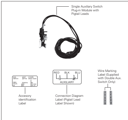
Fig. 2-1. Auxiliary Switch Kit
