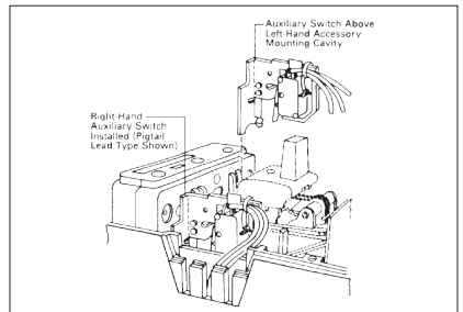
Fig. 2-3. Auxiliary Switch Installation Positions
