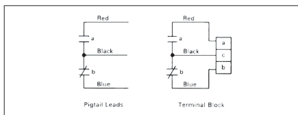
Fig. 2-6. Auxiliary Switch Connection Diagram
