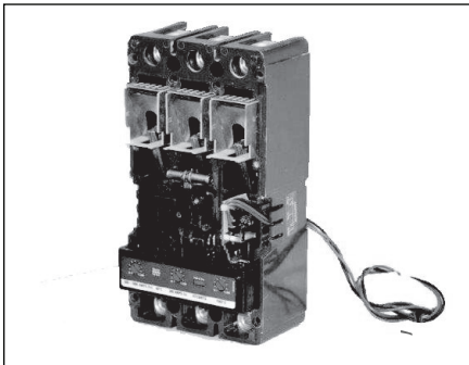
Fig. 1-1 Auxiliary Switch Installed in K-Frame Circuit Breaker
