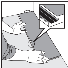
Fig.1 First plank, first row. Start in the left-hand corner of the room with the groove side of the locking profile facing you. Use a spacer (equal to the thickness of the floor) between the left wall and the plank. The spacers between the long sides and the wall will be added after three rows have been installed.
