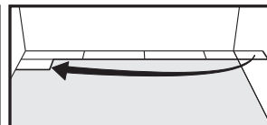
Fig.7 Second row. Utilize the leftover cut piece from the first row if it is 9" or longer. Hold the board at a 45-degree angle to the first board in the first row. Engage the boards' long sides, insuring they are completely engaged before rotating down while pushing it against the first board. If properly engaged, the boards will lie down flat. The gentle use of a tapping block may be helpful. Take care to not damage the locking system.
