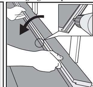
Fig.15 Put glue along the modified locking profile, press the panels together and weight until glue is dry.
