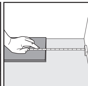
Fig.5 At the end of the first row, put a 3/8" spacer along the wall, measure the length of the last plank to fit.
