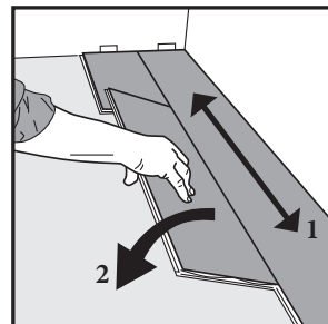
Fig.10 Hint for installing planks. The long sides of planks must be fully aligned before rotating down. You cannot force the boards. If they are not lying flat, the long side is not fully engaged. Start over ensuring the long sides are fully engaged.
