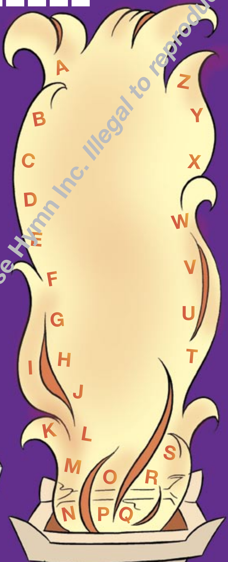
WORD SACRIFICES
