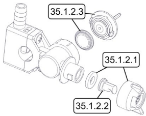
Center Nozzle Assembly
