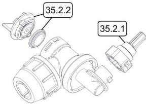
End Nozzle Assembly
