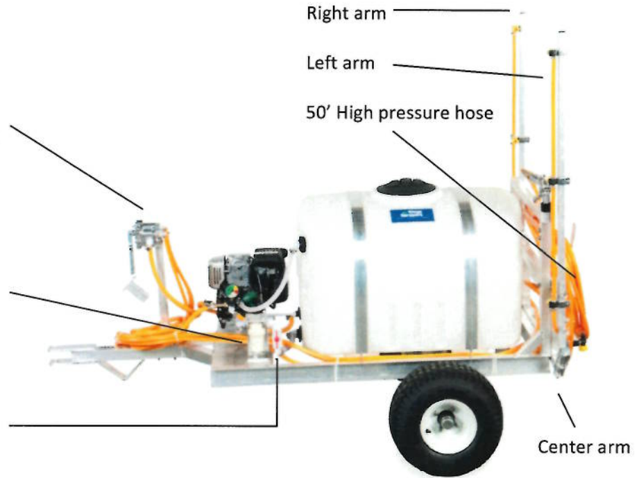
Figure 1: Side View
