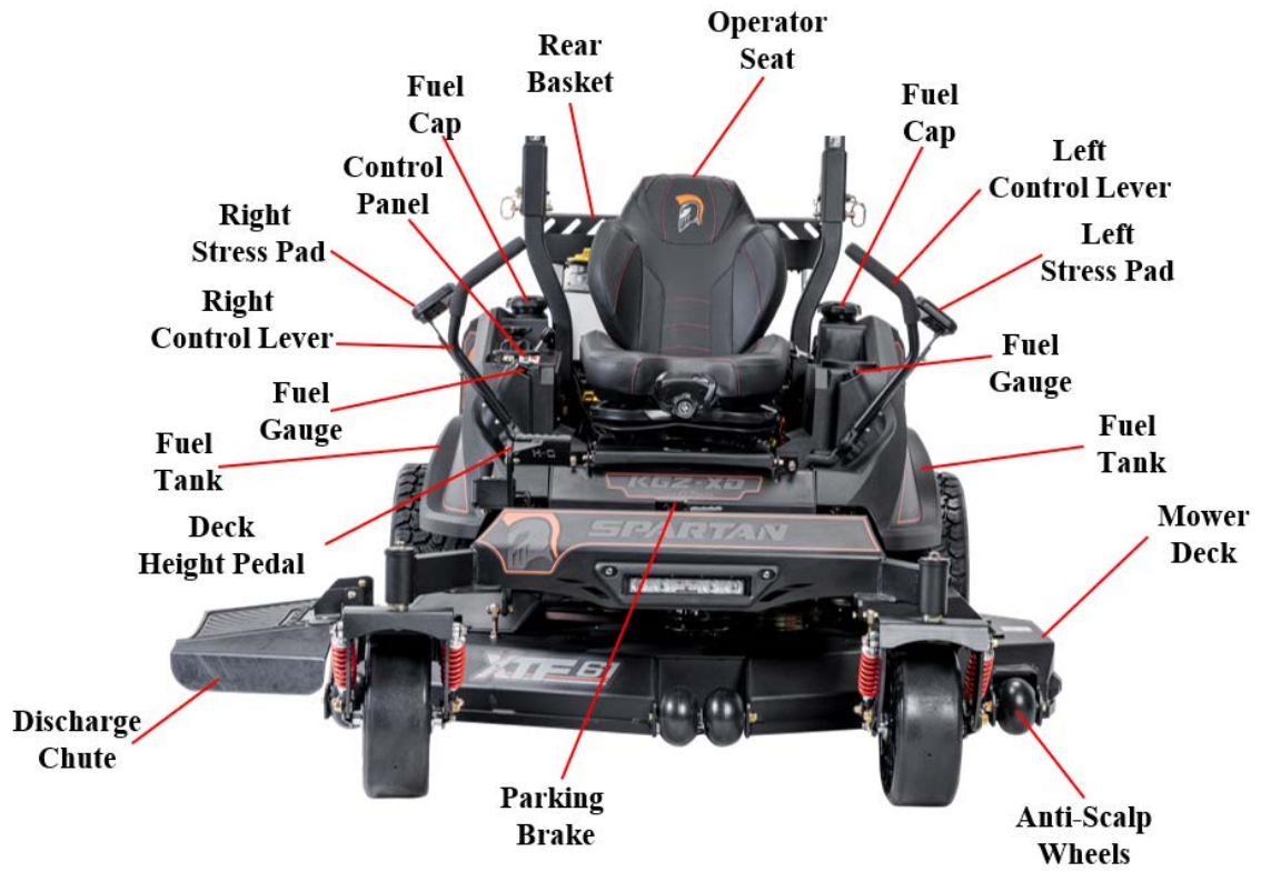
Figure 3.4: Front View
