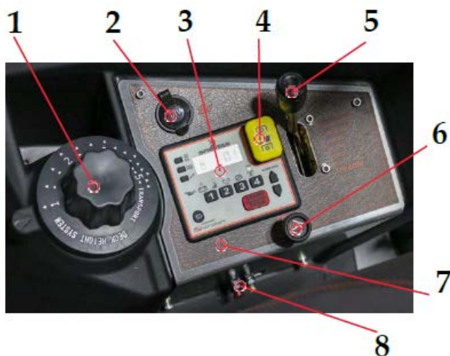
Figure 4.0 Operation Console
