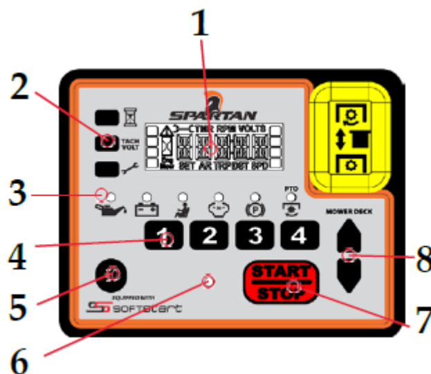
Figure 4.1: VersaGuard Console
