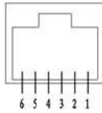
Figure 6. ST-4 Compatible Guiding Port Wiring
