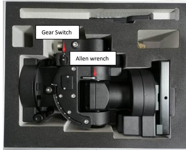
Figure 11. Remove the mount
