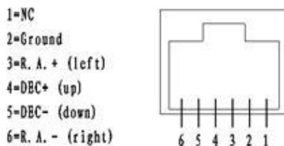
Figure 25. ST-4 port wiring
