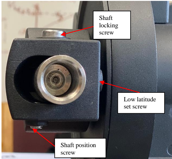
Figure 18. Screws for CW shaft tilting
