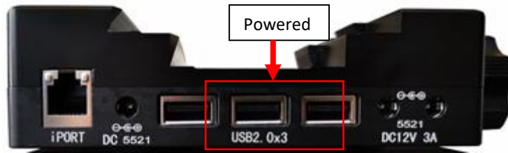
Figure 3. Ports on CEM70 dovetail saddle
