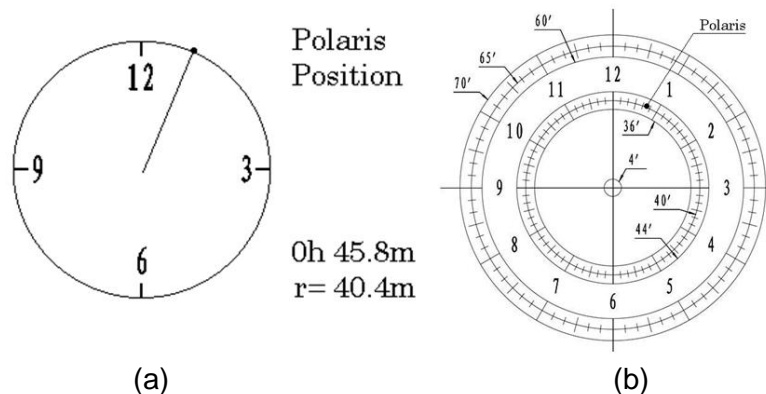
Figure 30. Polaris Position shown on HC (a) and where to put on polar scope dial (b)
