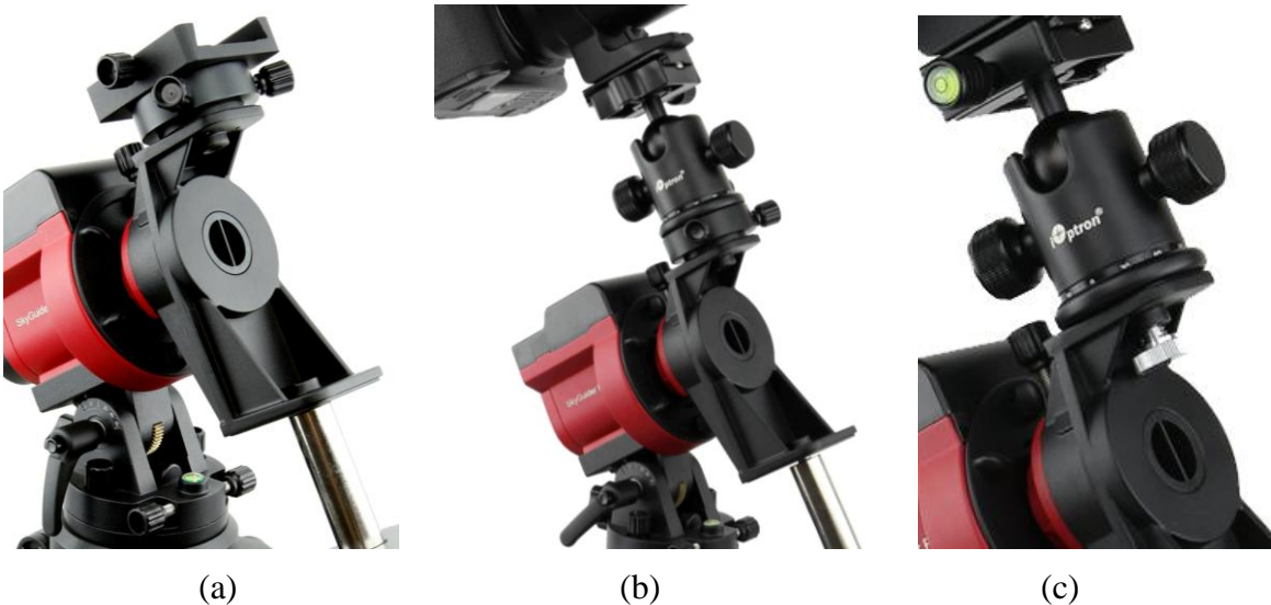
Figure 16. Various mounting methods
