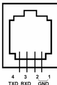
Figure 28. Serial port pin out on an 8408 hand controller
