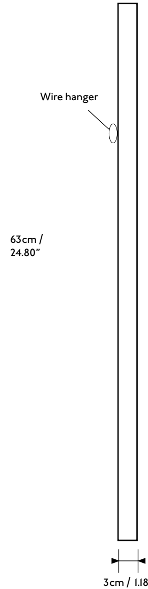
Side View
