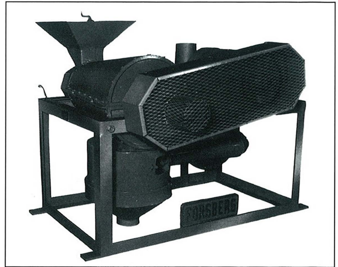
Model 2 Huller/Scarifier
