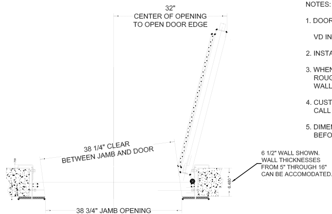
PLAN VIEW IN OPENED POSITION WITH CLEARANCE DIMENSIONS NOTED
