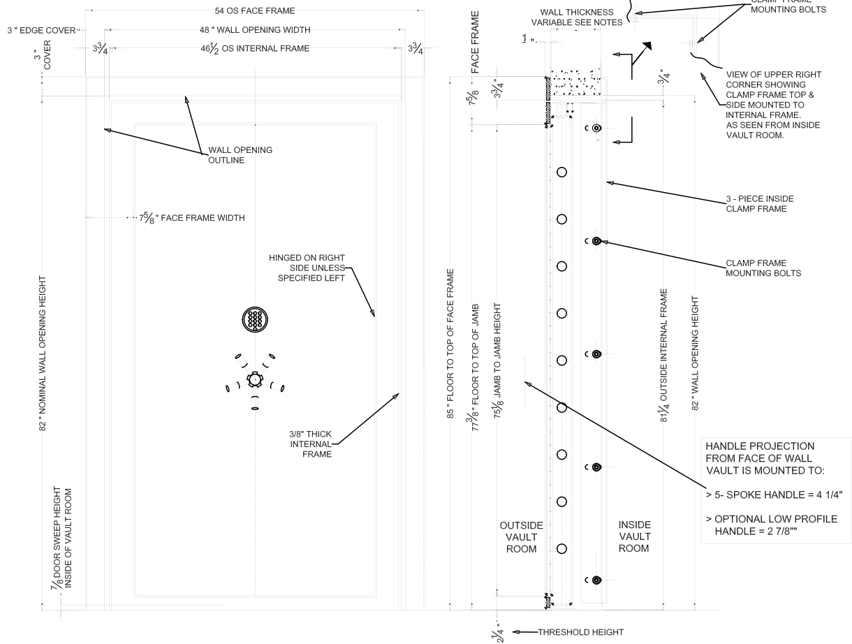
VD INSIDE SWING 8248 VAULT DOOR ELEVATION VIEWED FROM OUTSIDE
