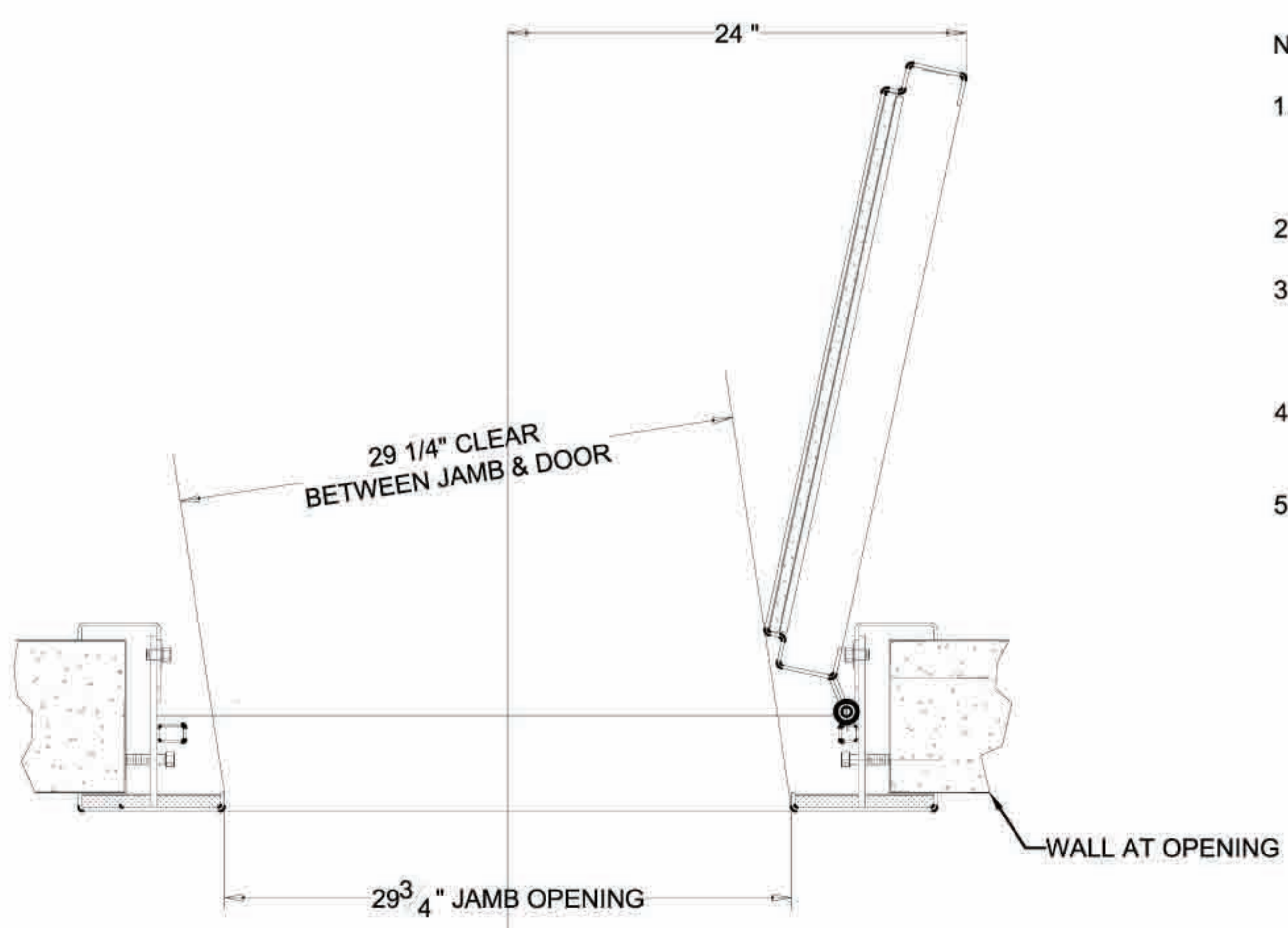
PLAN VIEW IN OPENED POSITION WITH CLEARANCE DIMENSIONS NOTED
