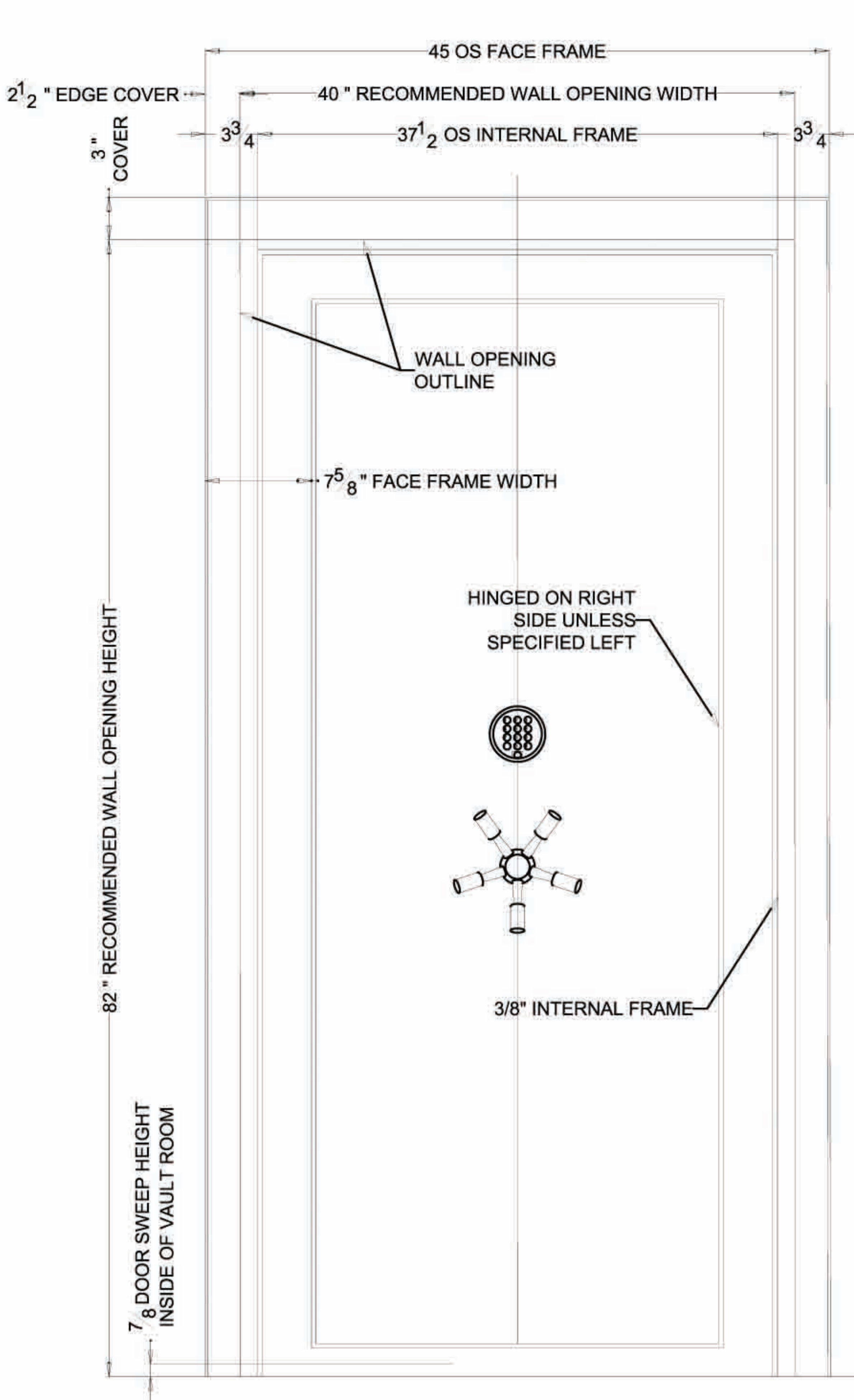
VD INSIDE SWING 8240 VAULT DOOR ELEVATION VIEWED FROM OUTSIDE
