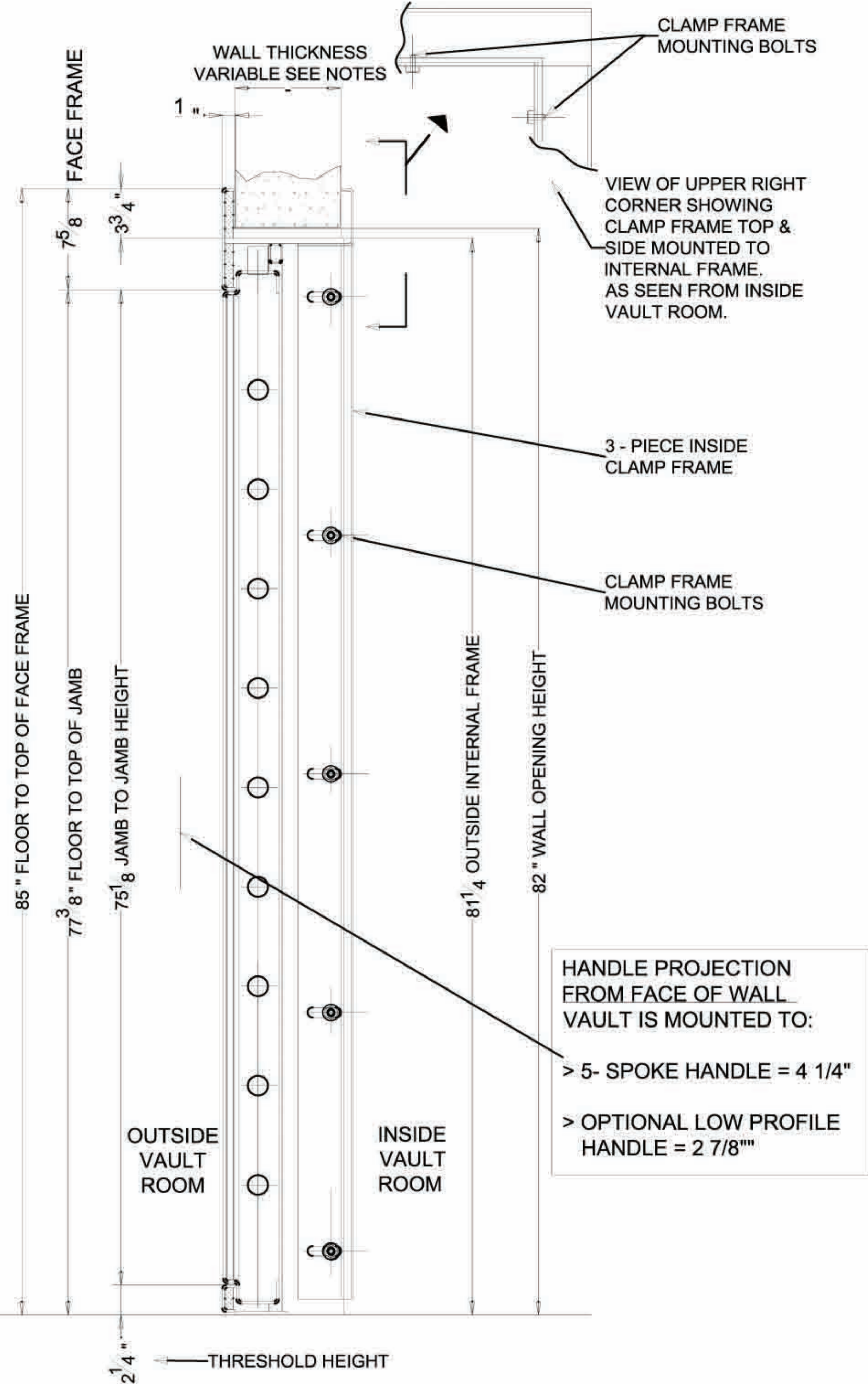
SECTIONAL SIDE VIEW OF FRAME
