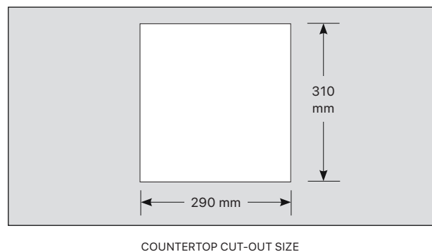
COUNTERTOP CUT-OUT SIZE
