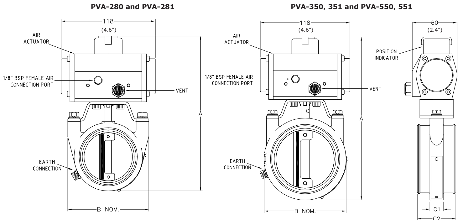
Dimensions in mm (inches)
