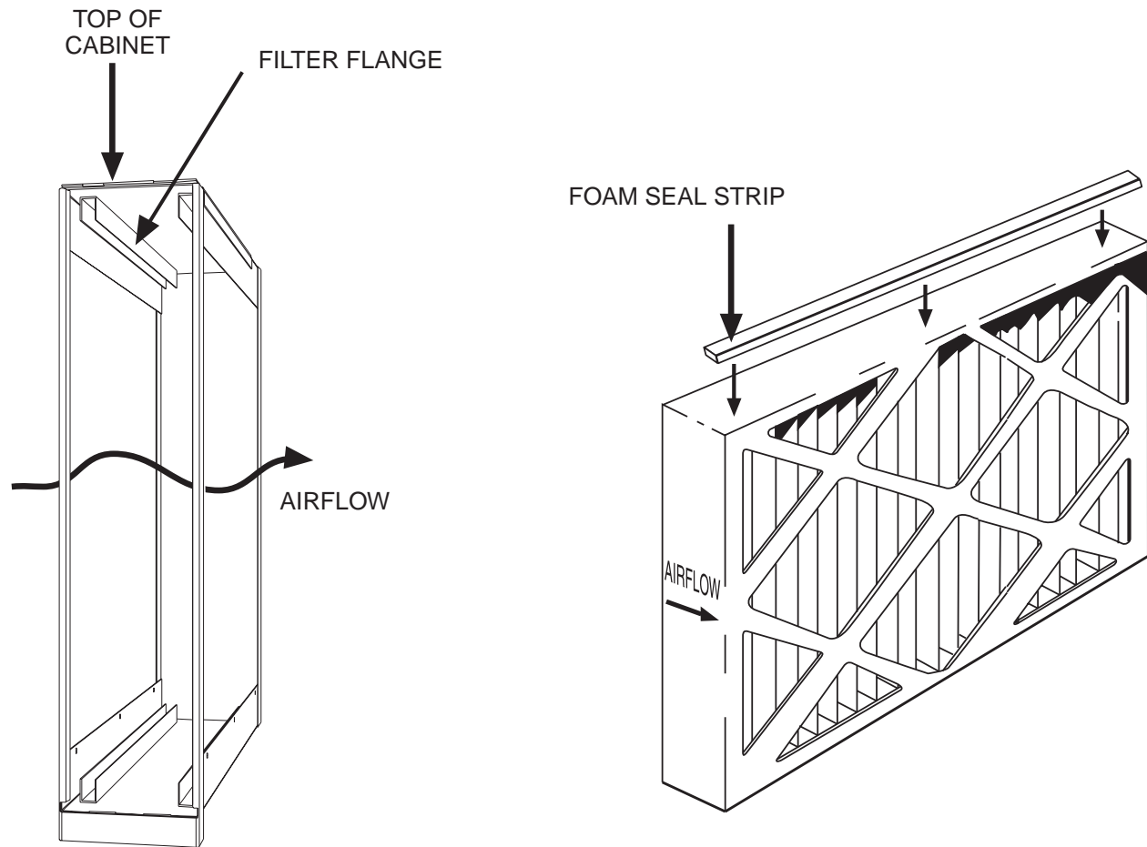
Fig. 1—Typical Seal Strip Installation
