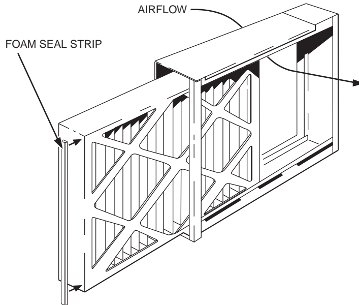
Fig. 2—Seal Strip Installation in MPKA Cabinet (and large Honeywell cabinets)
