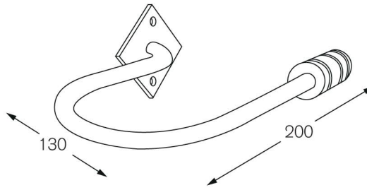
Dimensions for all Metal Holdbacks (available with every finial except Stooper and Spear)
