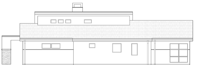
LEFT ELEVATION
