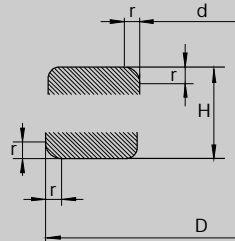
Fig. 6-3 One-Way Thrust Ball Bearings
