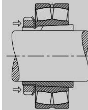
Fig. 14-5 Mounting on an Adapter Sleeve
