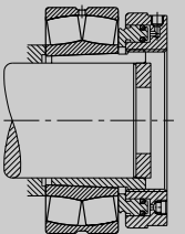
Fig. 14-13 Dismounting of Withdrawal Sleeve by using Hydraulic Nuts
