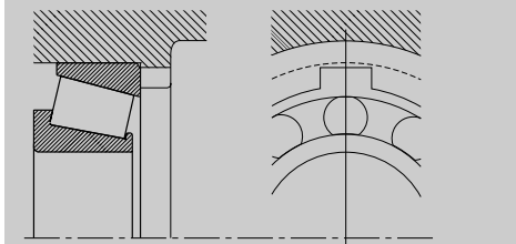
Fig. 14-17 Dismounting Groove
