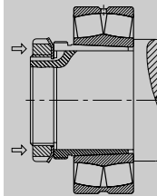
Fig. 14-6 Mounting on a Withdrawal Sleeve
