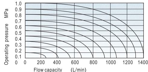
Model: CM3B-08
