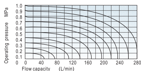
Model: CM3B-06
