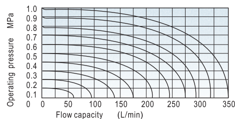
Model: CM3B-08
