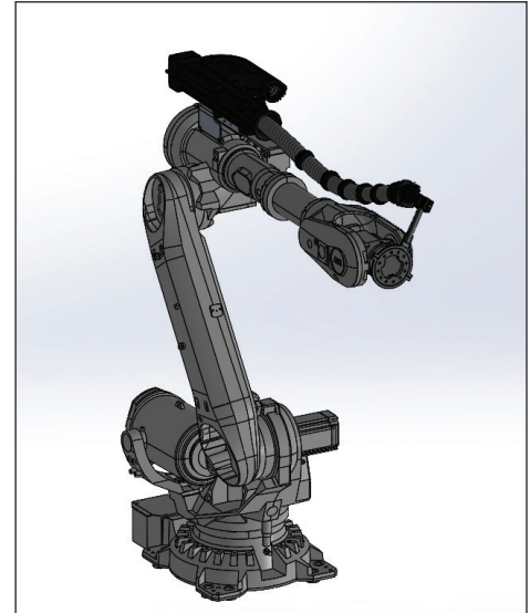
26.70.321.01 Complete robotic dresspack, Axis 3-6, TecBox retraction system, 600mm stroke, high-flex conduit with ID 64mm
