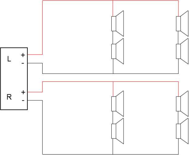
series-parallel wiring (8Ω/channel)
