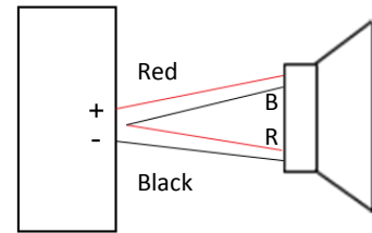
Series bridged/mono wiring ( 16\Omega )
