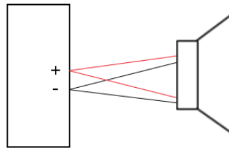
Parallel bridged/mono wiring ( 4\Omega )
