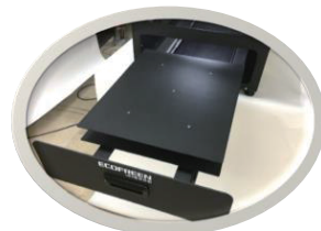
40x50cm (16"x20") Size Platen Thick hood jacket can be loaded
