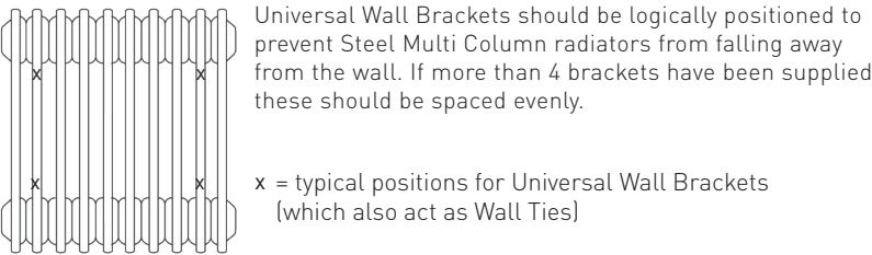
Fig 1 - Bracket Positions
