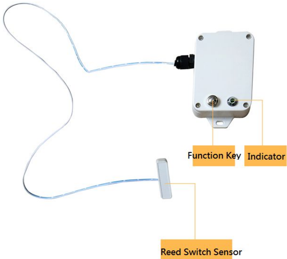
Fig.1 R718F Appearance
