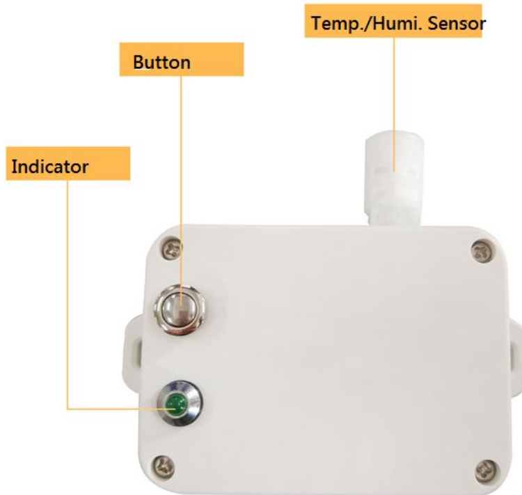
Fig.1 R718AB Appearance
