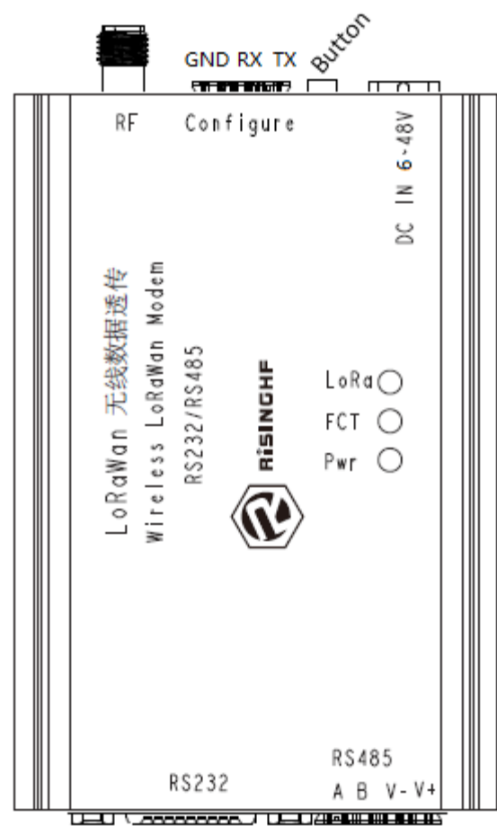
Figure 3-2 RHF3M485 interface
