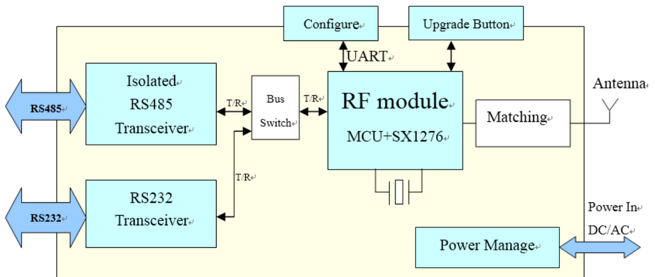
Figure 3-1 Block Diagram of RHF3M485
