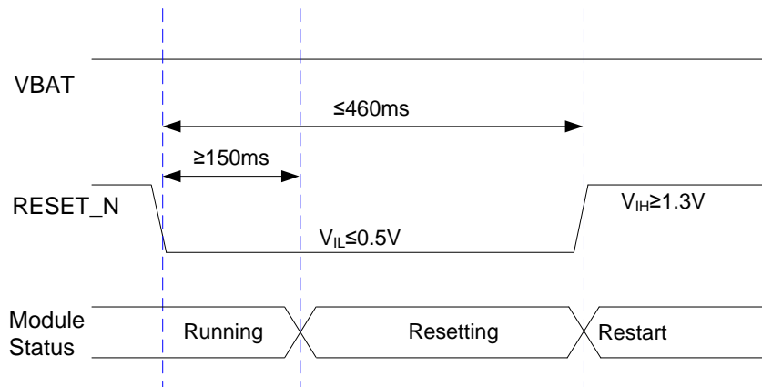
Figure 16: Reset Scenario of Module
