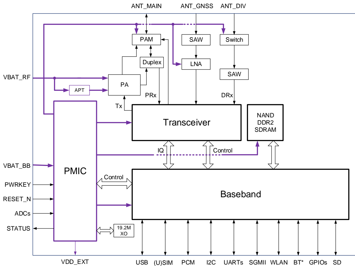
Figure 1: Functional Diagram
