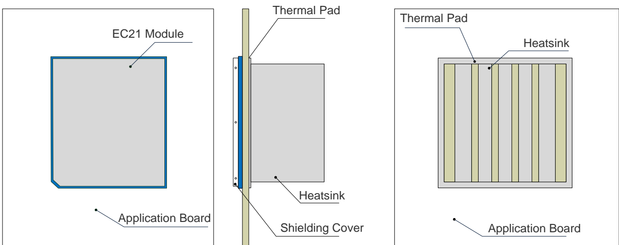
Figure 43: Referenced Heatsink Design (Heatsink at the Bottom of Customers' PCB)
