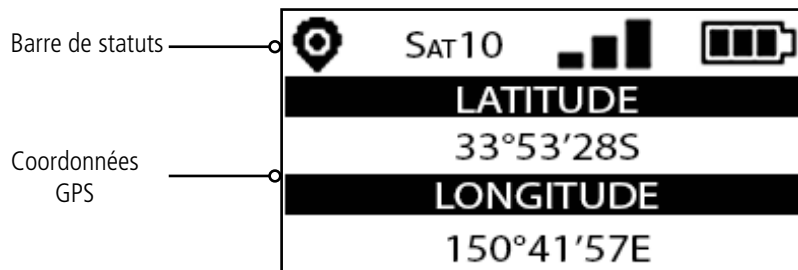
Figure 9 : Ecran GPS
