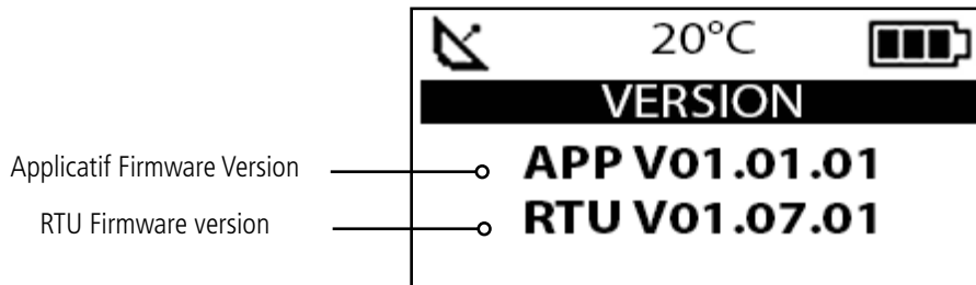
Figure 5 : Firmware version
