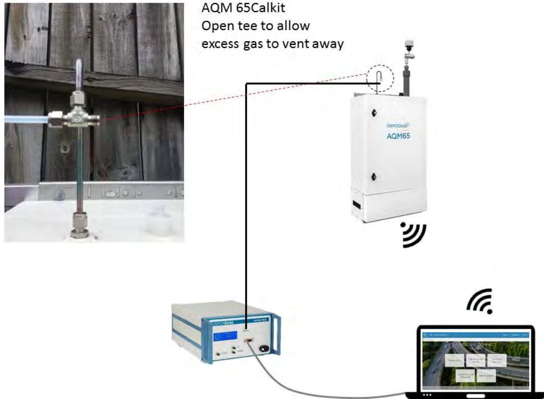
Figure 5-11 Setup to perform zero calibration with AirCal 1000
