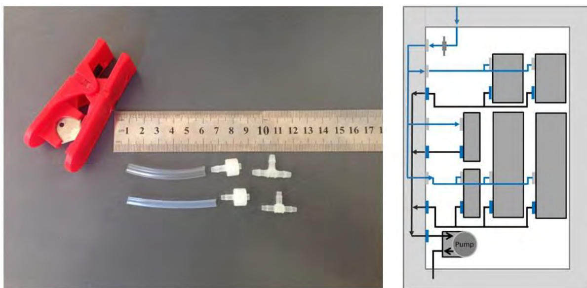
Figure 4-27 Adding a new module requires adding additional sample and exhaust lines.
