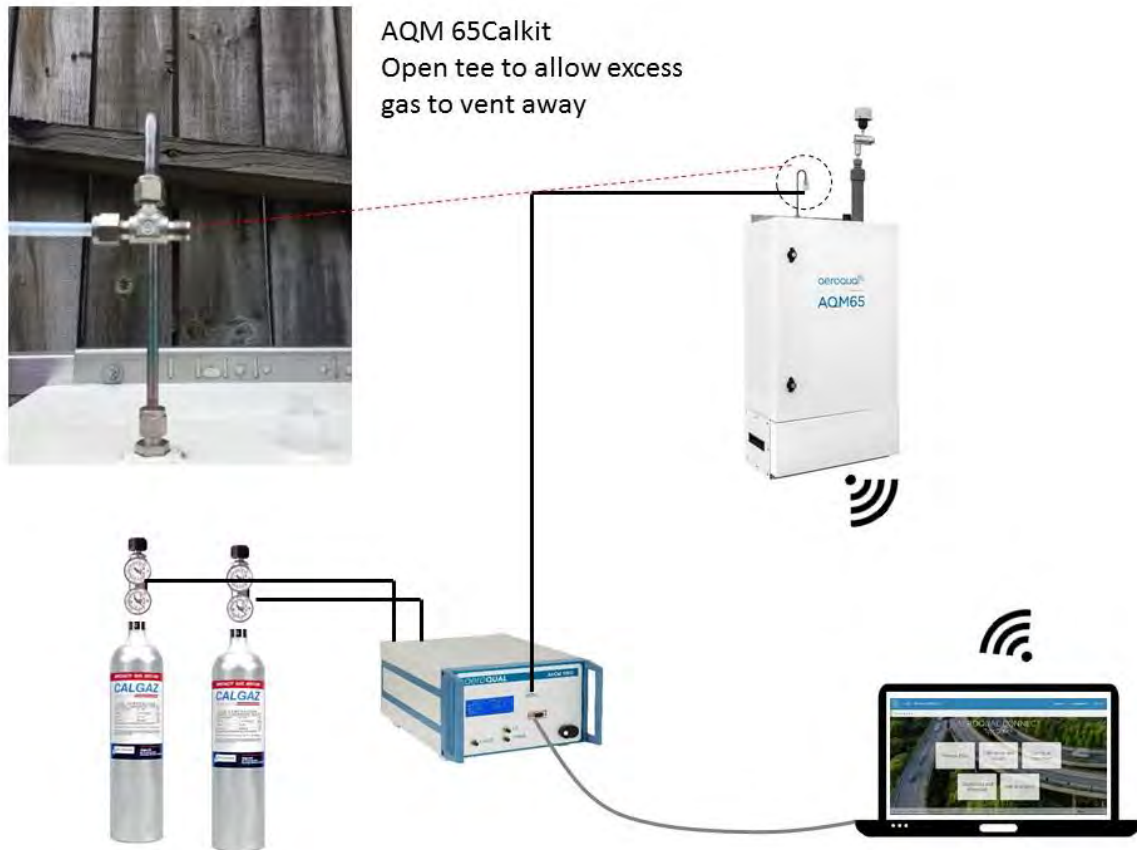
Figure 5-12 Setup to perform span calibration with AirCal 1000
