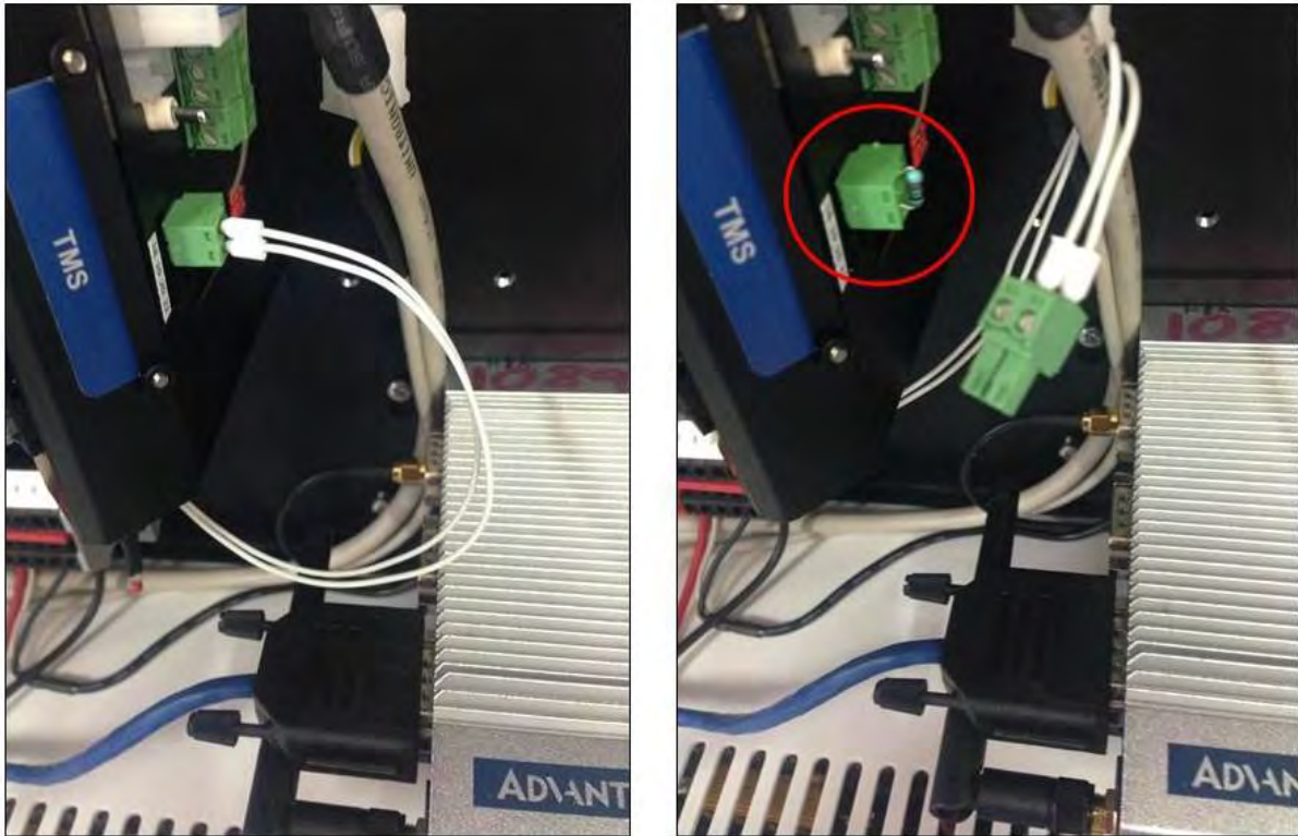
Figure 4-34 Replace the internal temperature sensor with the temporary plug shown
