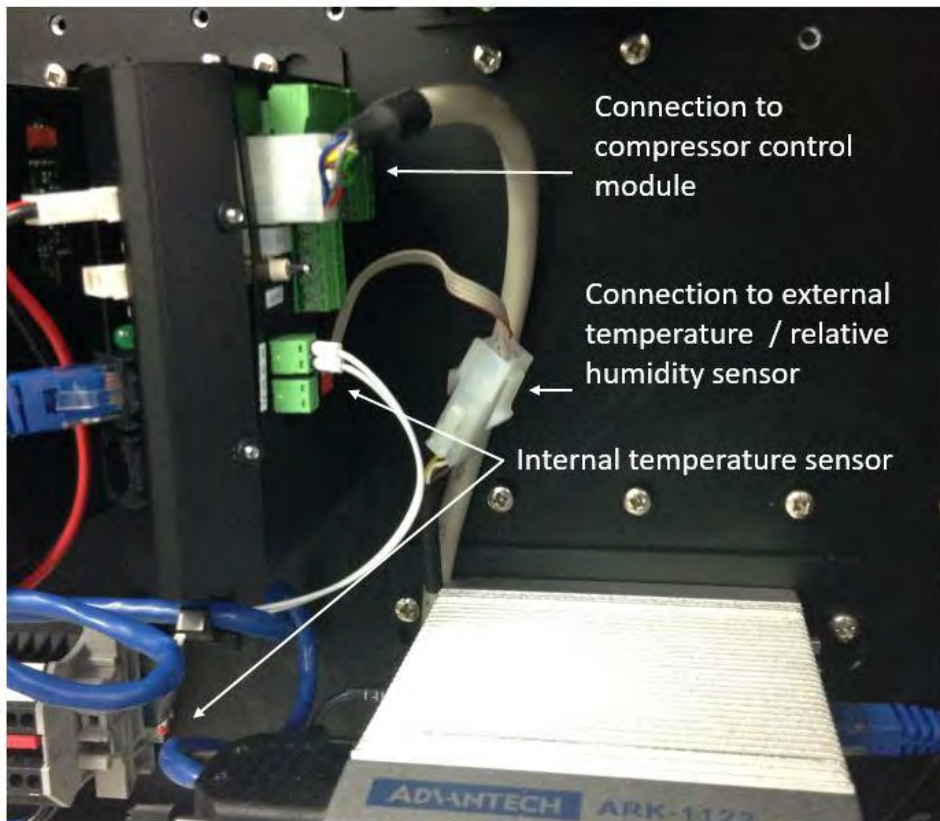
Figure 1-21 The system manager module controls the internal temperature and also measures the external temperature and relative humidity
