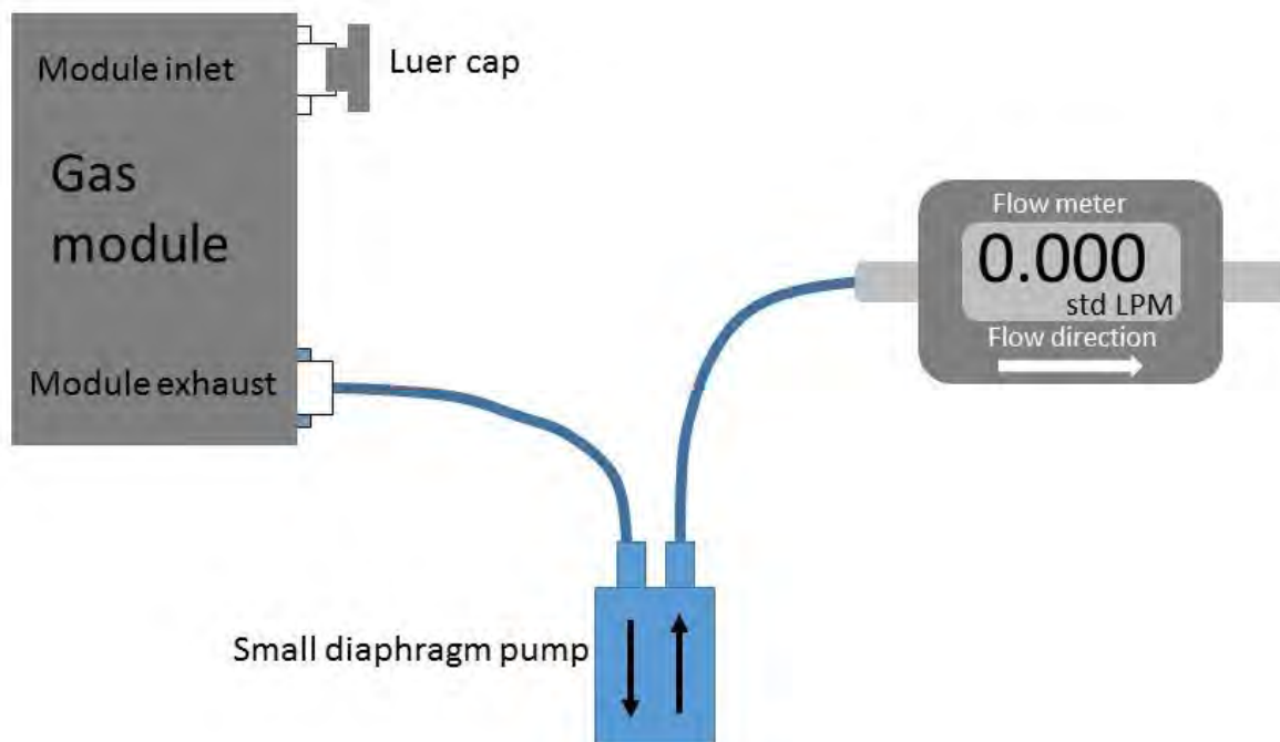
Figure 4-24 A gas module can be checked for leaks by using a diaphragm pump and R7 flow meter
