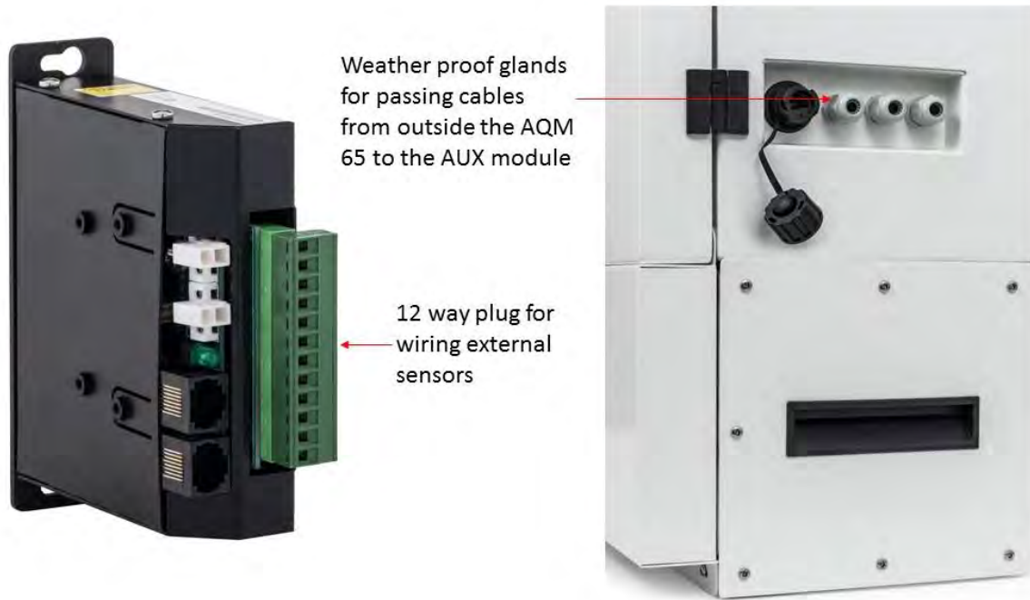
Figure 1-19 The external sensors are connected to the green plug on the Aux module. The cable passes through water proof glands on the right wall of the AQM 65
