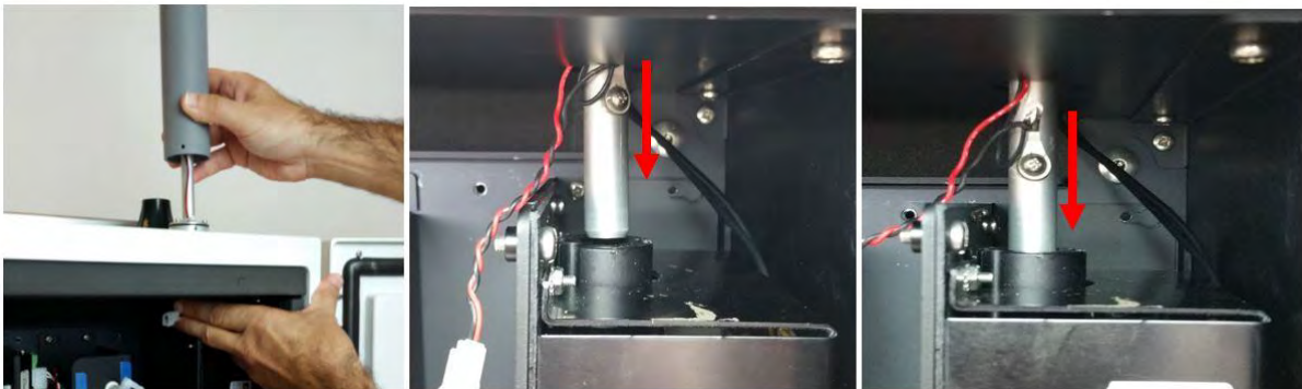
Figure 2-7 Gently feed in the power cable. The aluminium tube must push all the way in to the PM module.
