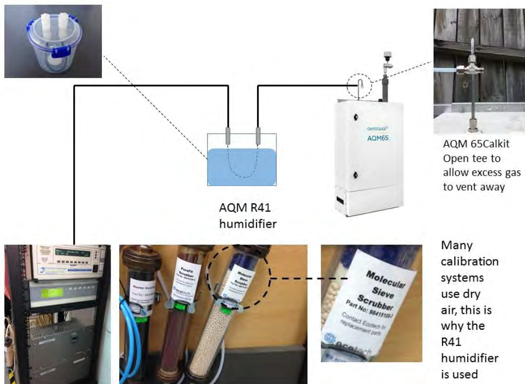
Figure 7-4 The Aeroqual R41 humidifier is placed between the outlet of the calibrator and the inlet of the AQM 65
