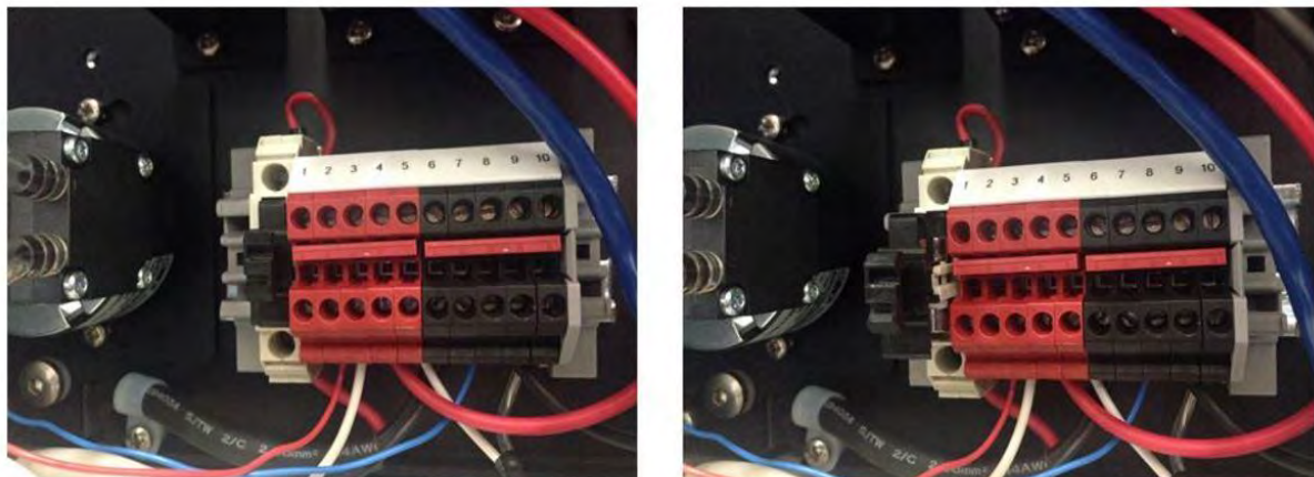
Figure 2-3 The 12V DC fuse can be pulled out to turn off the AQM or pushed in to power the AQM 65
