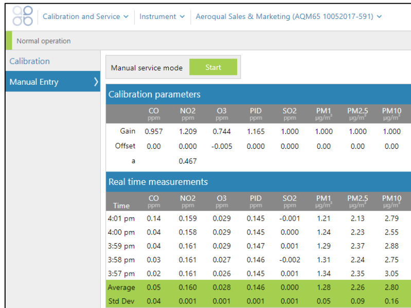
Figure 5-15 The Manual Entry screen of the Calibration and Service app
