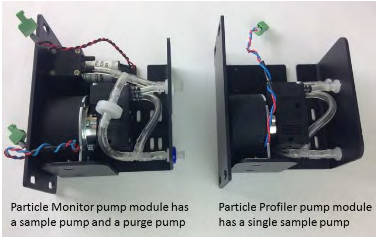
Figure 4-23 The Particle Monitor contains two pumps; the Particle Profiler has one pump
