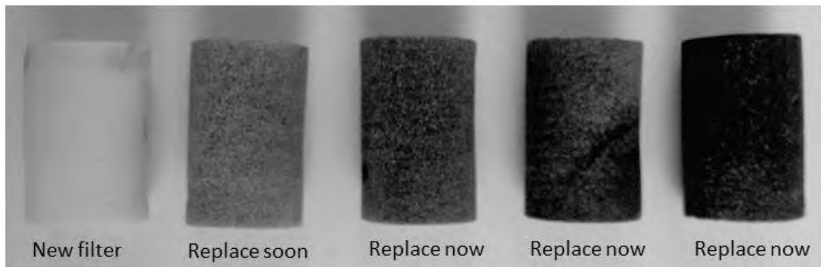
Figure 4-9 The AQM R31 sample filter should be replaced once the filter begins to blacken
