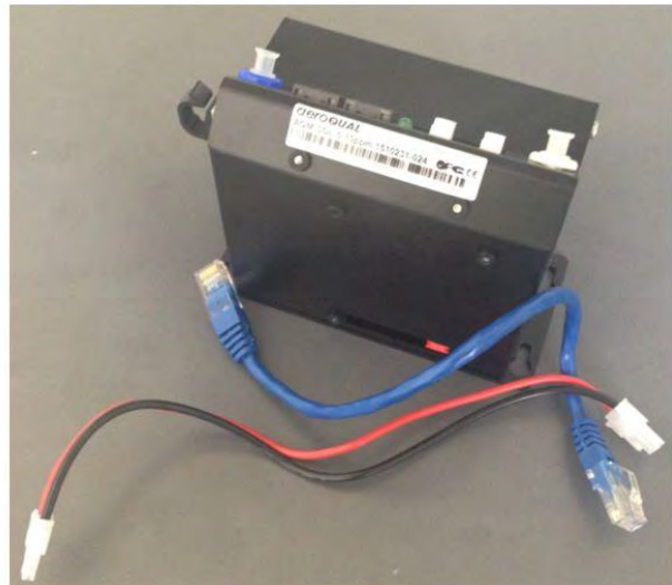
Figure 4-26 When removing a module, cap the gas lines. You should also remove one communication lead and one power lead.
