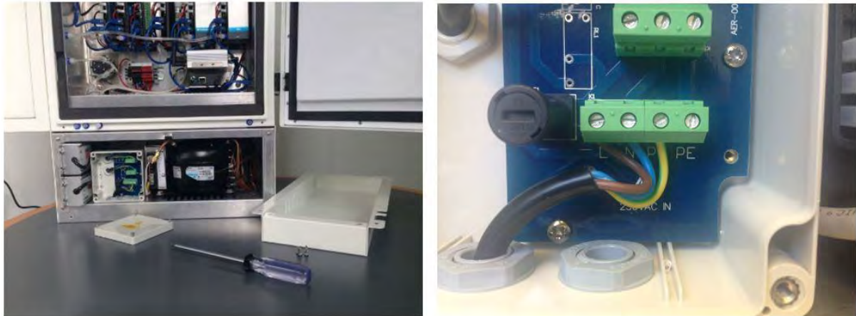
Figure 2-2 Remove the front cover to wire mains power to the AQM 65
