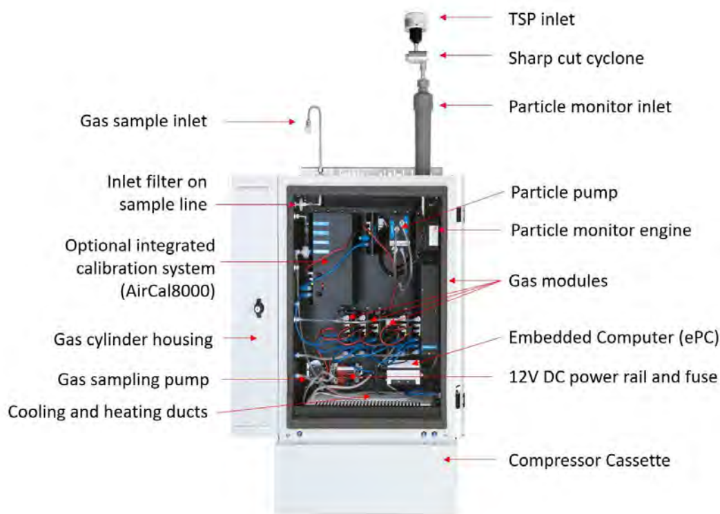
Figure 1-1 AQM 65 with key parts labelled
