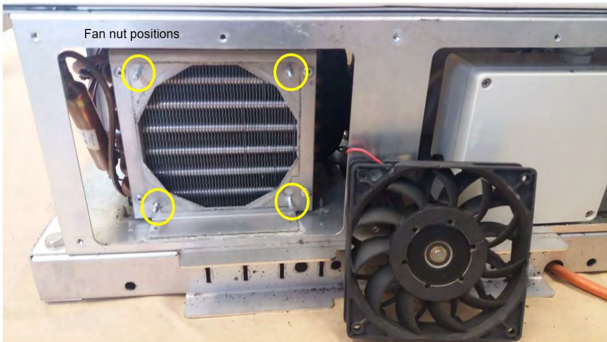
Figure 4-31 The cooling can be removed for cleaning. Make a note of the orientation of the fan and replace back the fan in the same position
