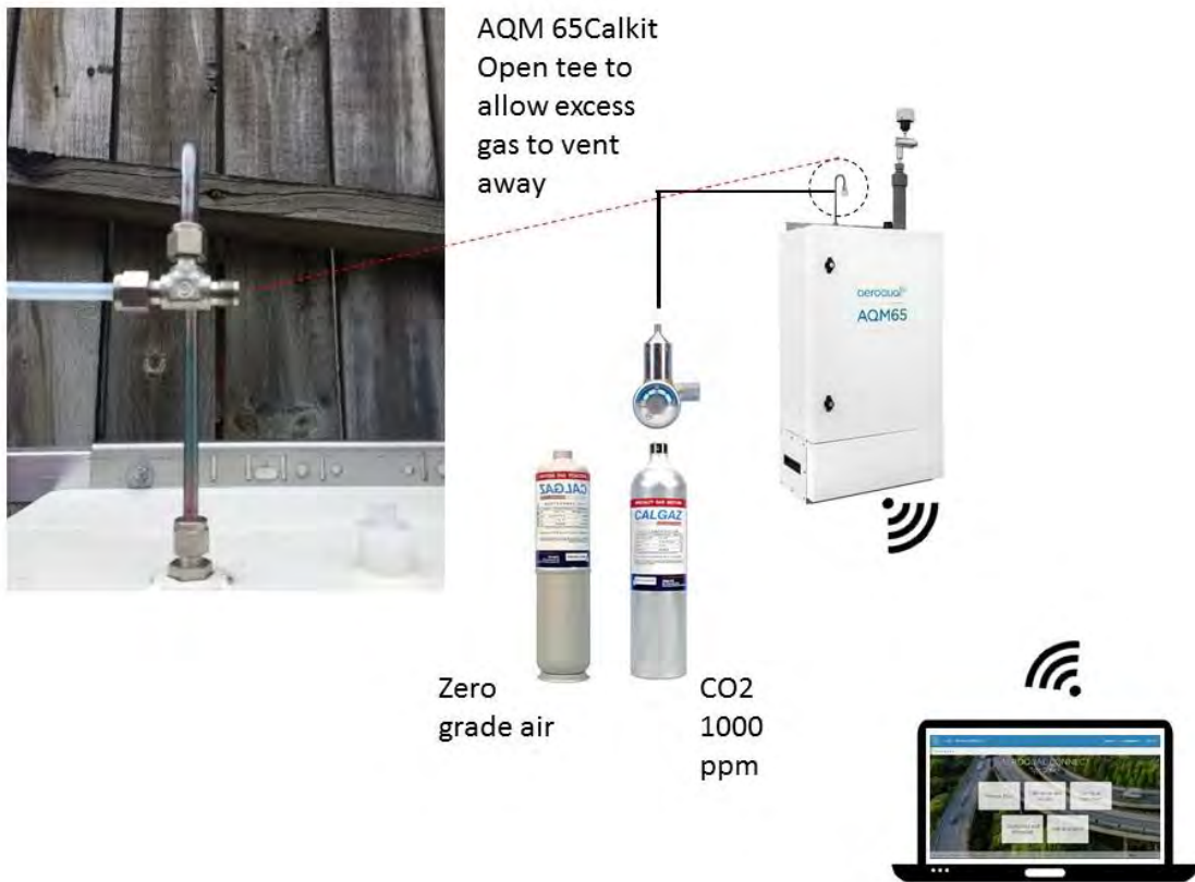
Figure 7-1 Calibration setup for calibrating CO2
