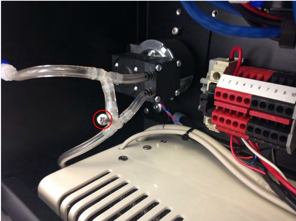
Figure 4-7 The flow adaptor valve is used to adjust the AQM 65 inlet flow to the correct value.
