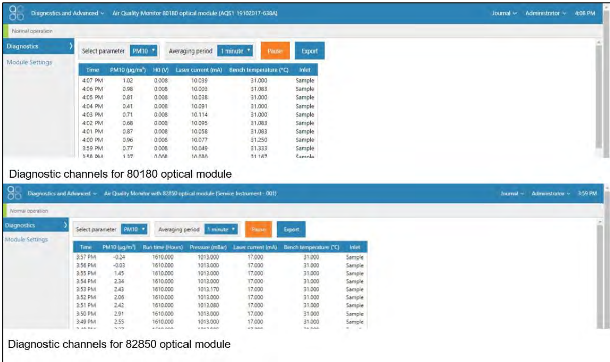
Figure 4-20 Comparison of diagnostic channels between 80180 and 82850 optical modules
