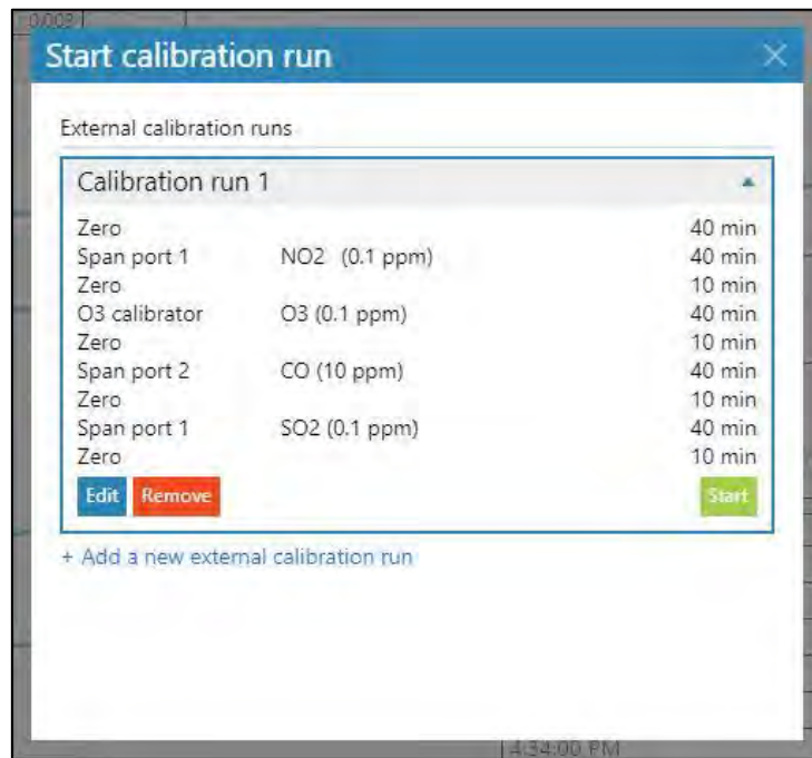
Figure 5-17 The calibration run configurator
