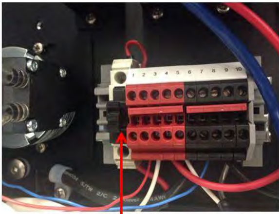
12 V DC fuse pushed in, the “on” position
