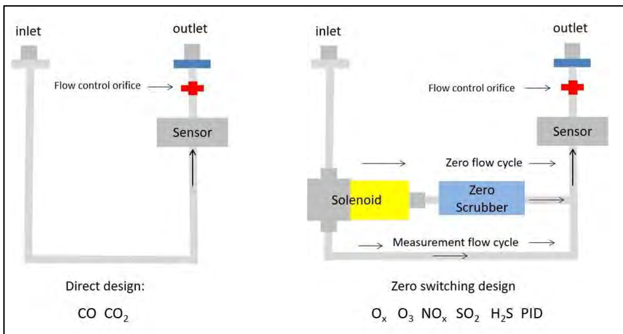
Figure 1-2 Gas sensor modules are based on two different designs
