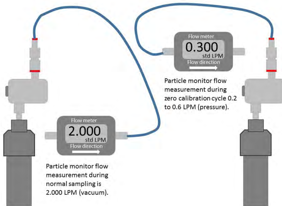
Figure 4-18 When measuring the sample flow of the Particle Monitor a vacuum is measured. When measuring the zero flow a positive pressure is measured.
