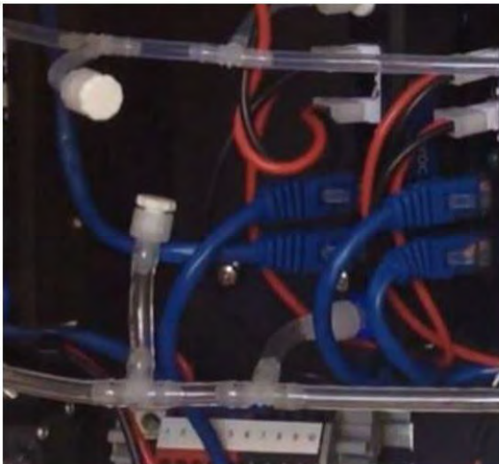
Figure 4-26 When removing a module, cap the gas lines. You should also remove one communication lead and one power lead.
