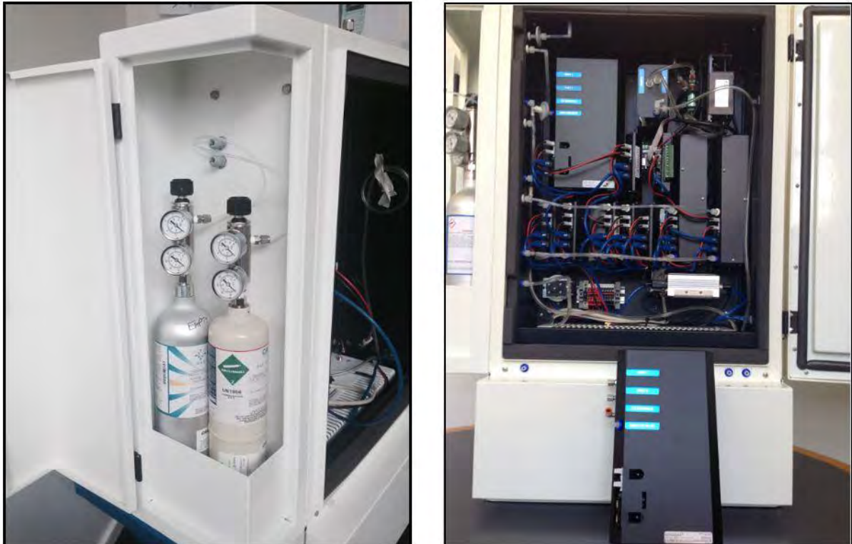
Figure 5-5 The AirCal 8000 stores calibration cylinders in a compartment on the left side. All of the components required to perform the calibration are in a module inside the AQM 65.
