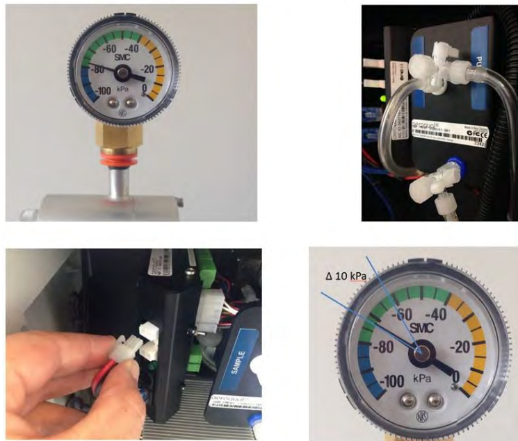
Figure 4-14 Fit the vacuum gauge, adjust the valves. Then stop the pump by removing power from the module, observe the change in pressure. If the leak rate is greater than 10 kPa in 10 seconds then there may be a leak in the system. Check all the tube connections.
