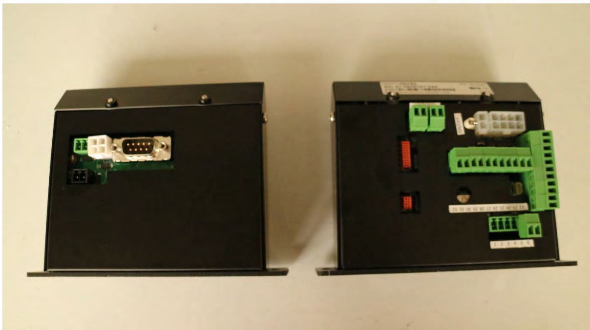
Figure 1-14 Left IO module for the 82850 optical module, note that the fibre span switch is no longer used, Right IO module for the 80180 optical module
