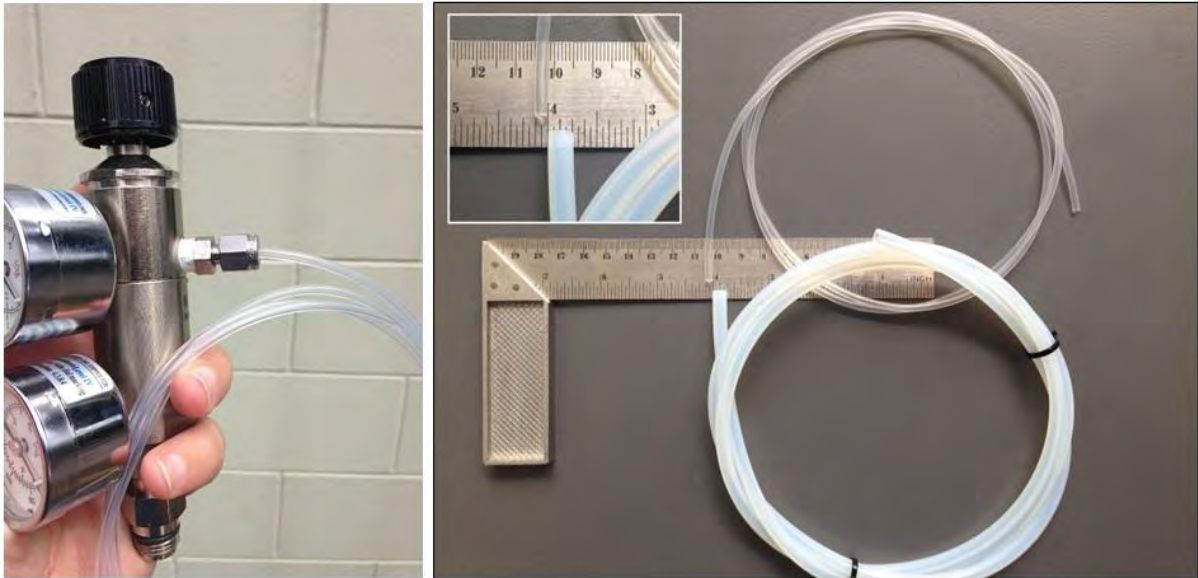
Figure 5-7 The Aeroqual gas regulator is fitted with a 1/8 inch Swagelok compression fitting. Additional tubing for calibration can be purchased from Aeroqual: 1/8 OD tube Aeroqual part number CS Tube 27 and 1/4 OD Tube Aeroqual part number AS R66.
