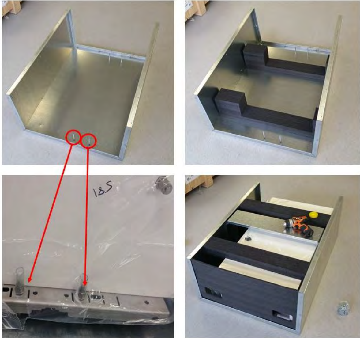
Figure 2-14 The packing crate uses retaining bolts which go through the AQM 65 mounting brackets. There is an additional supporting brace shown in the top right image which should be used.
