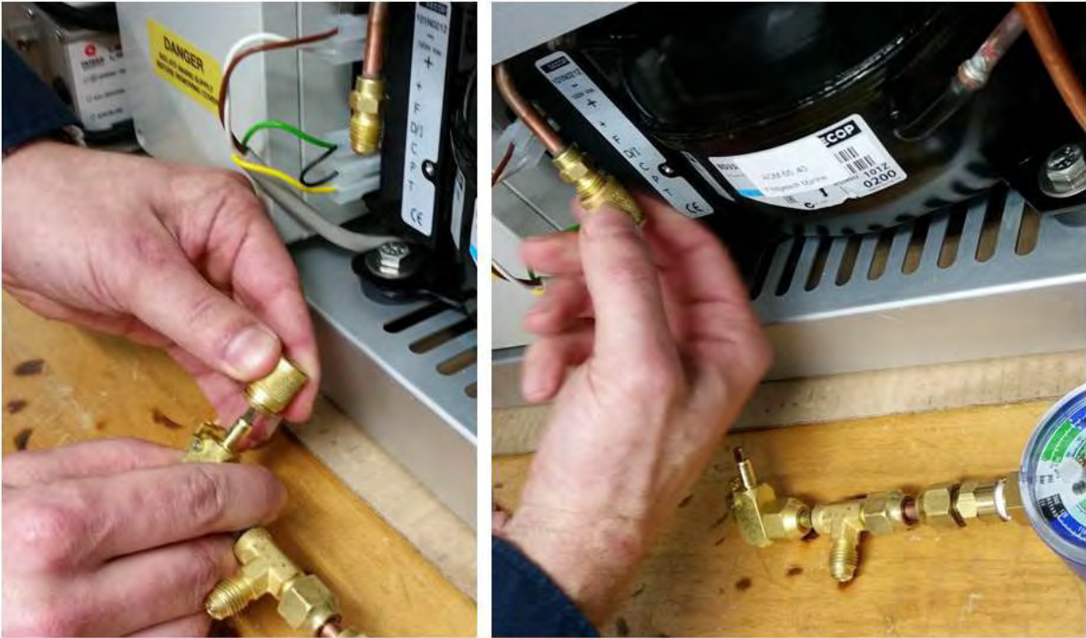
Figure 4-36 Attach the charging cap from the pressure gauge and screw it on to the gas inlet on the compressor
