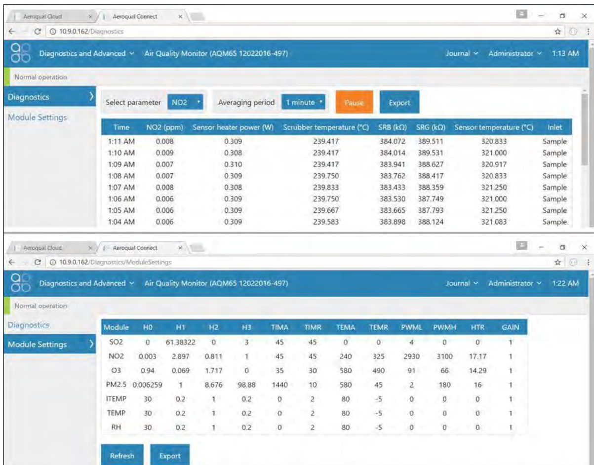
Figure 3-15 The Diagnostics and Advanced app displays real time instrument operational readings and settings which control how the modules are controlled.
