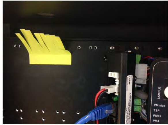
Figure 2-4 With mains power on, and with the 12 V DC fuse pulled out, there should be air flow coming from the top of the AQM as shown on the right. Disconnect the power (red/back) cable from the PM pump module while testing the power, as shown on the left
