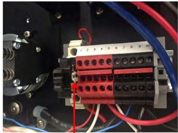
12 V DC fuse pulled out in the “off” position
