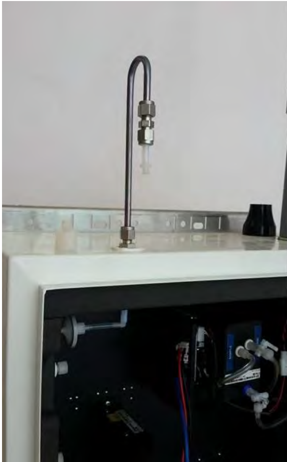
Figure 4-5 To measure the flow rate, remove the inlet filter and attach the inlet flow adaptor.
