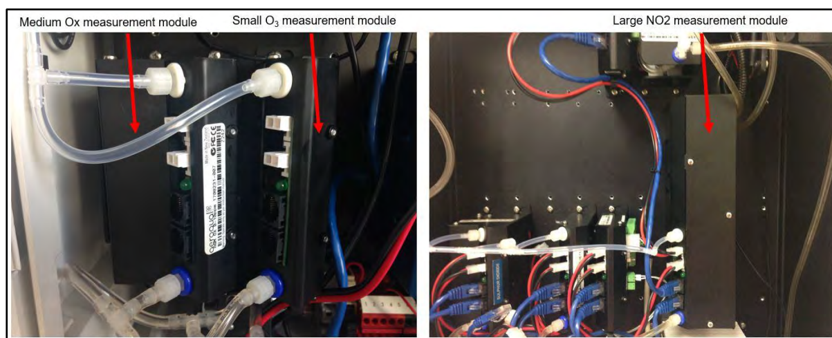
Figure 5-10 Left: An Ox measurement module and Ozone measurement module, (the power and communication cables have been removed for clarity). Right: NO 2 direct measurement module.
