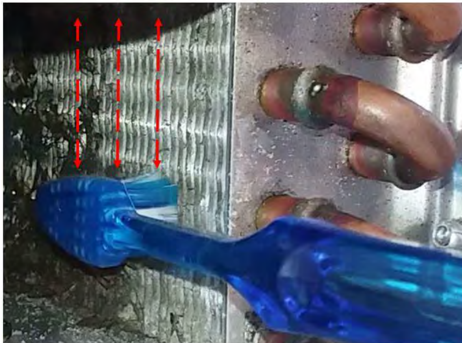
Figure 4-30 Clean the condenser fins by brushing up and down parallel to the direction of the fins
