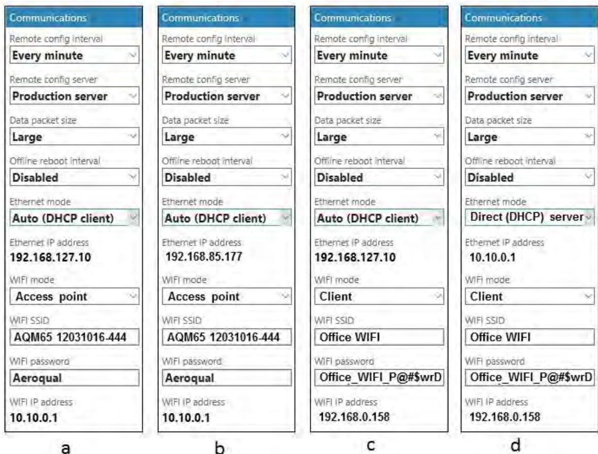
Figure 3-7 The different connection types require different settings in the Configure Instrument app
