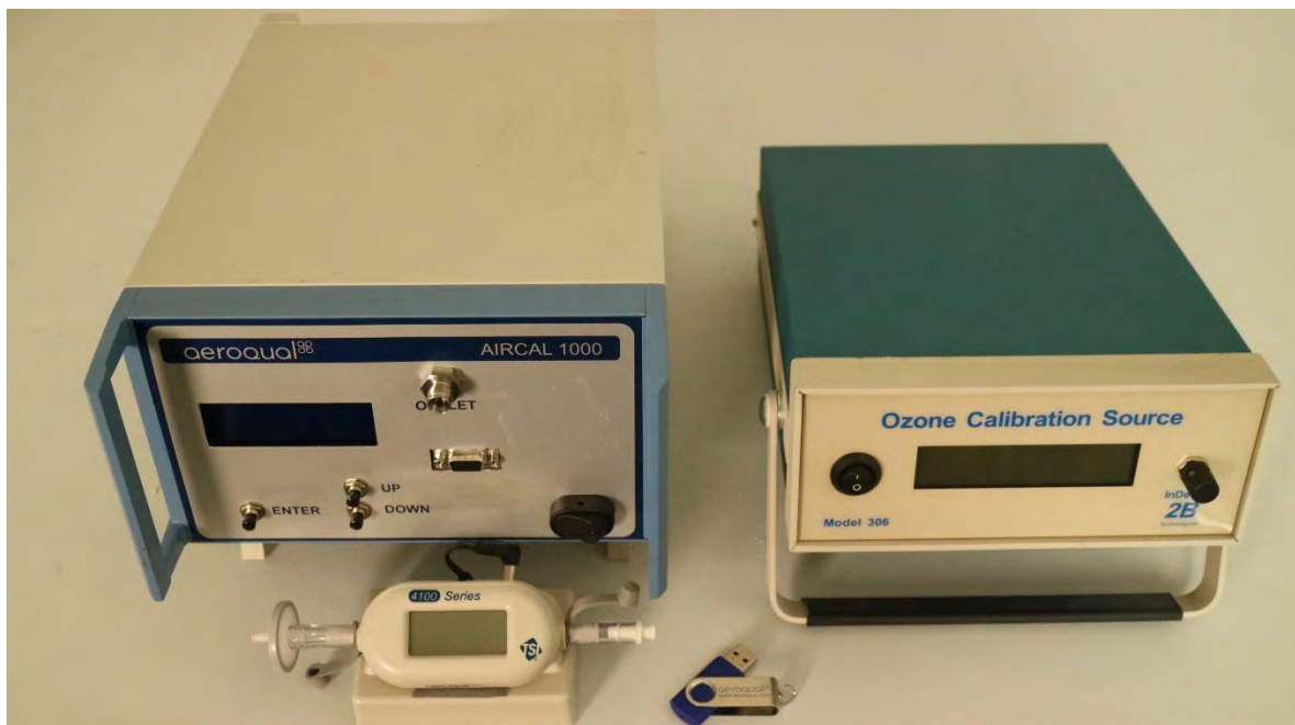
Figure 5-3 The Ozone calibrator (right) and AirCal 1000 (left) are light weight and can easily be transported to the AQM 65
