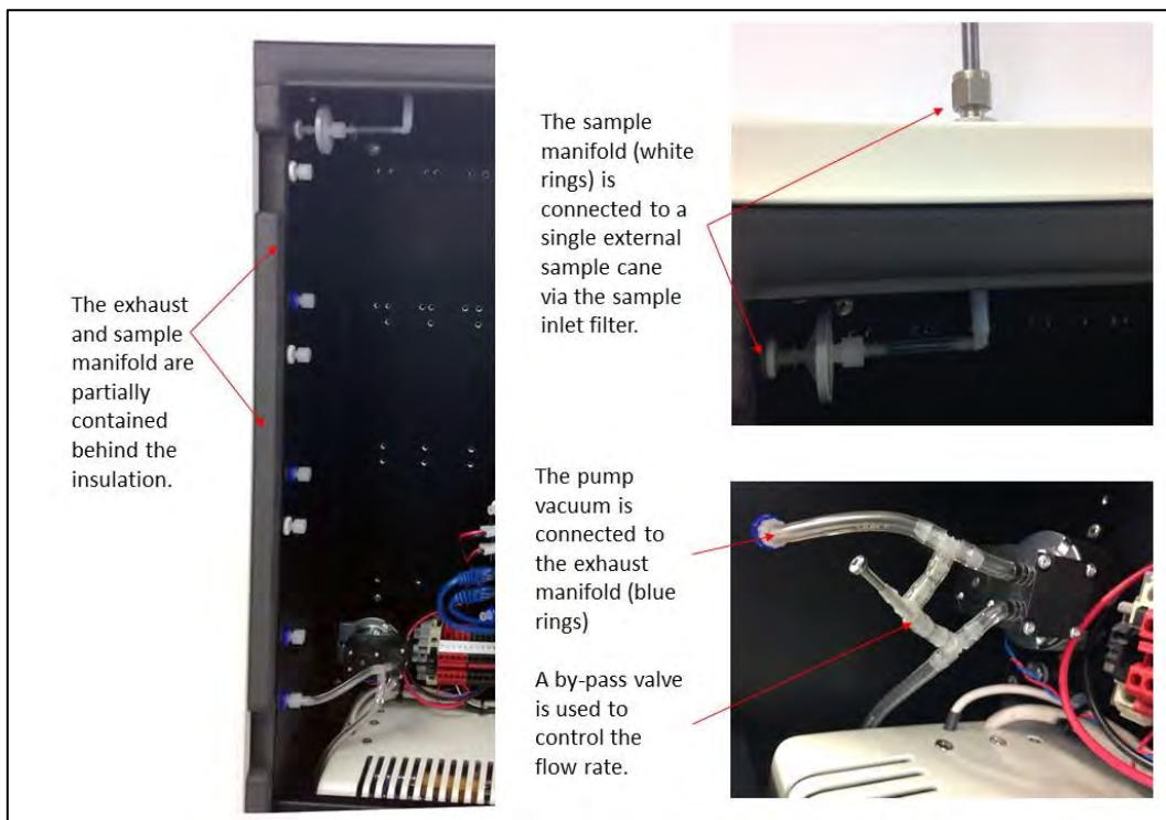
Figure 1-9 The vacuum side of the pump is connected to the exhaust manifold (blue rings). The AQM 65 inlet is connected to the inlet manifold (white rings). The pump has a by-pass valve to control flow rate.
