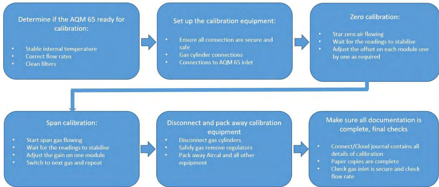
Figure 5-8 Flow schematic for calibration
