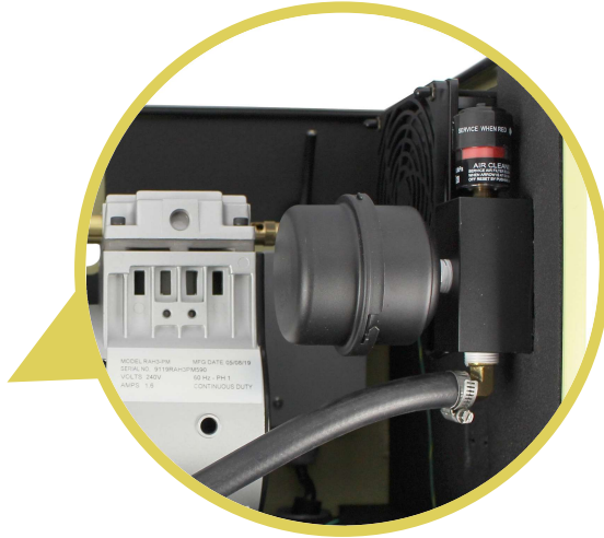
ABOVE: New visual maintenance indicator installed on air filter. When indicator turns red, filter maintenance is needed.
