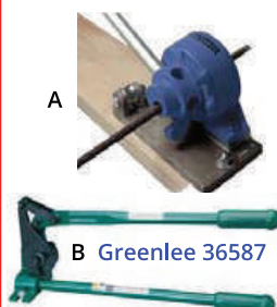
Rebar Bender-Cutters A Bender-Cutter up to 5/8" B Cutter only up to 3/8"
