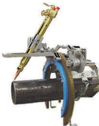
Pipe Beveling Machine and Torches
