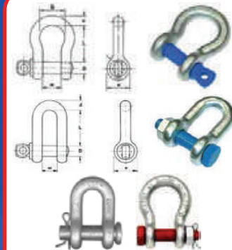
Shackles Pin & Screw Pin 3/16" to 2" Bow & Straight types
