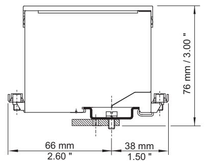
Safety barriers 9001, 9002, 9004 mounting on mounting plate by means of adaptor
