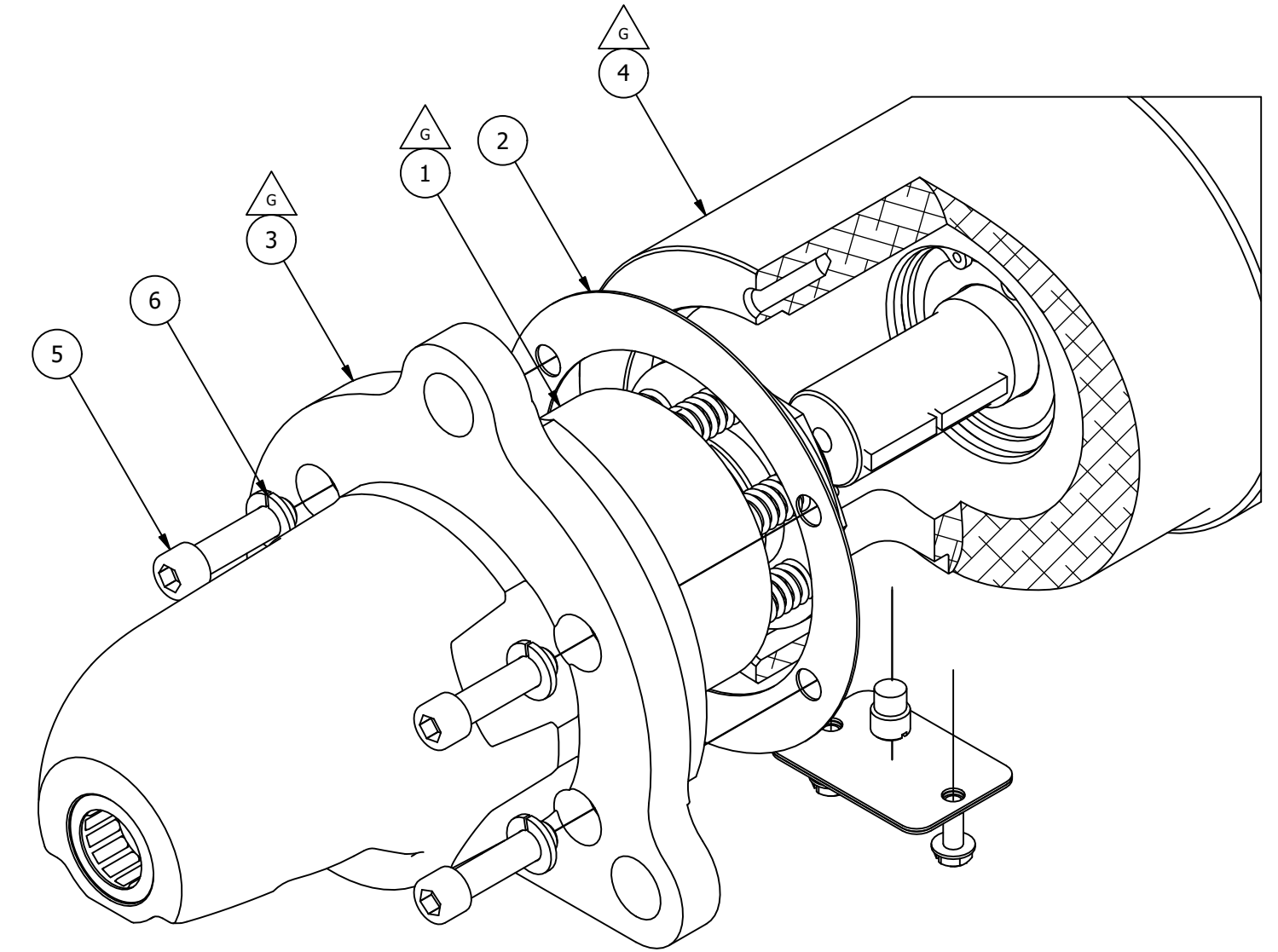
ASSEMBLY DETAIL VIEW SCALE: 0.65 : 1
