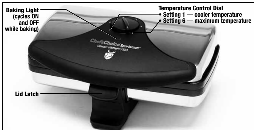
Figure 1. Classic WafflePro®.
