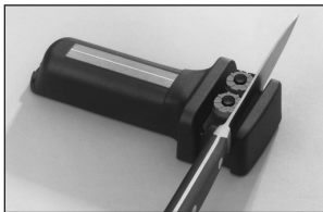
Figure 4: Sharpening in Stage 2.
