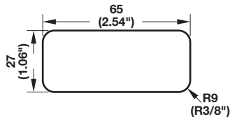
Cut-out Dimensions
