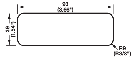
Cut-out Dimensions
