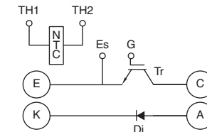
NX-Series Chopper IGBT CM200EXS-34SA
