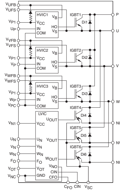
PSS05SA2FT, PSS10SA2FT, PSS15SA2FT, PSS25SA2FT, PSS35SA2FT, PSS50SA2FT
