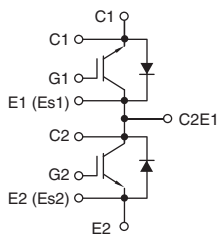
S-Series Dual AC Switch IGBT CM400C1Y-24S
