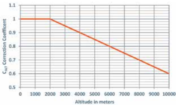
Graph 4: Altitude derating
