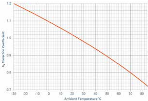
Graph 1: Temperature Correction
