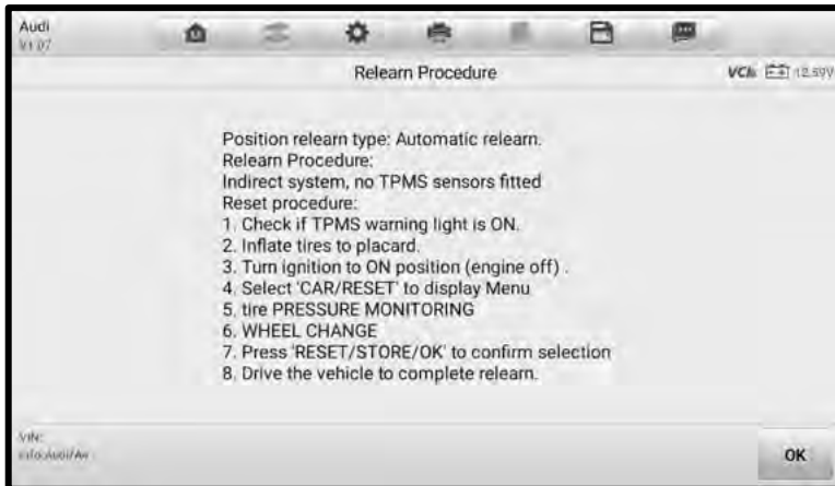
Figure 4-12 Relearn Procedure for Indirect TPMS
