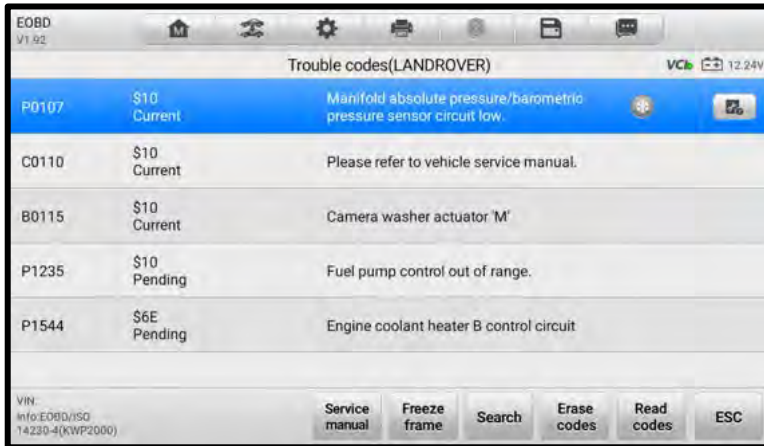
Figure 5-25 DTC & FFD Screen
