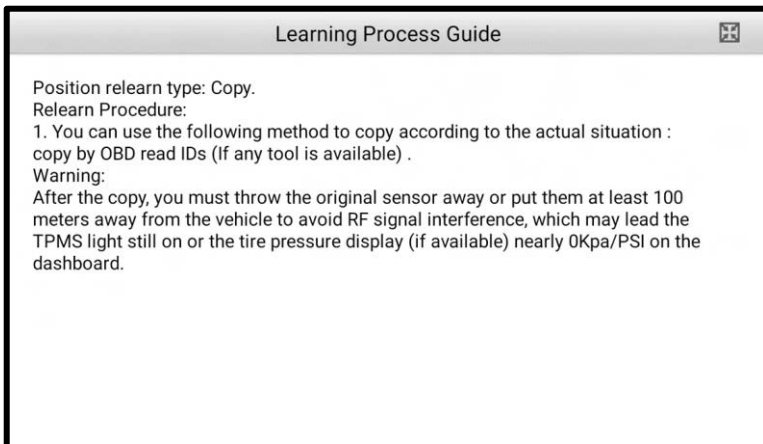
Figure 4-34 Copy Relearn Screen 2
