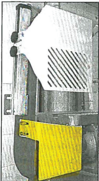
Fig. 1 Left hand mount and lower belt guard
