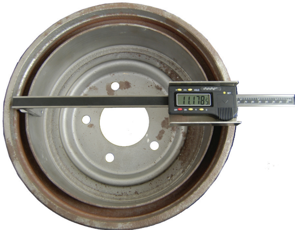
Shown Above: Internal Drum Diameter Measurement
