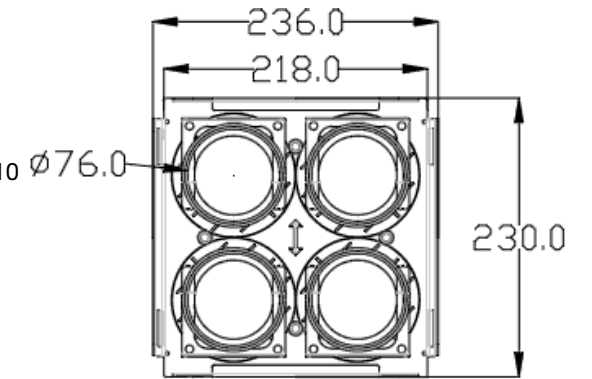
990 323 610 Top View
