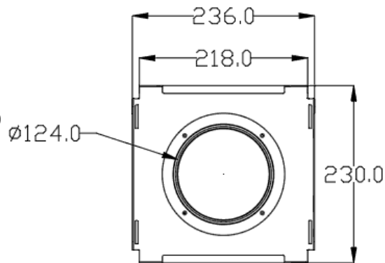
990 323 510 Top View
