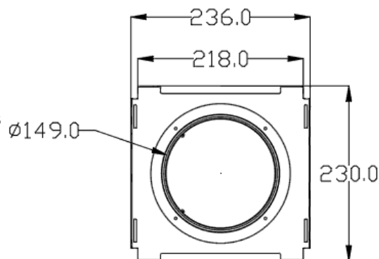
990 323 563 Top View
