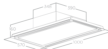
FALSE CEILING CUT: 550X980
