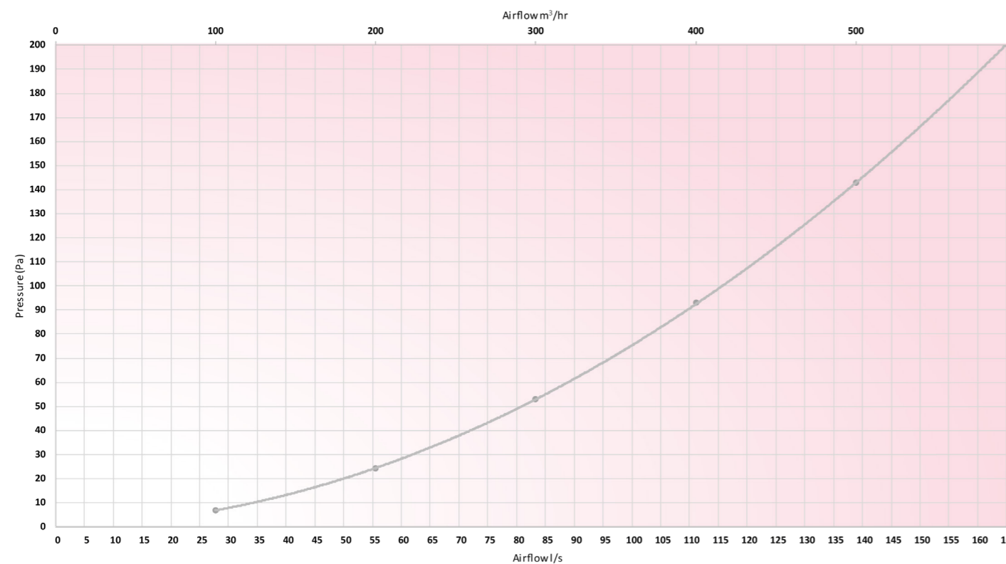
Plastic manifold, 1 x \varnothing 125mm connection, 5 x \varnothing 75mm ports
