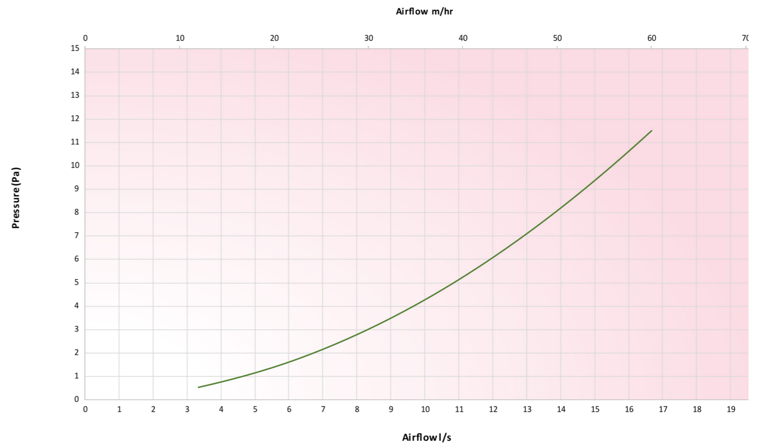
Zehnder ComfoTube ø 75mm, 90° bend
