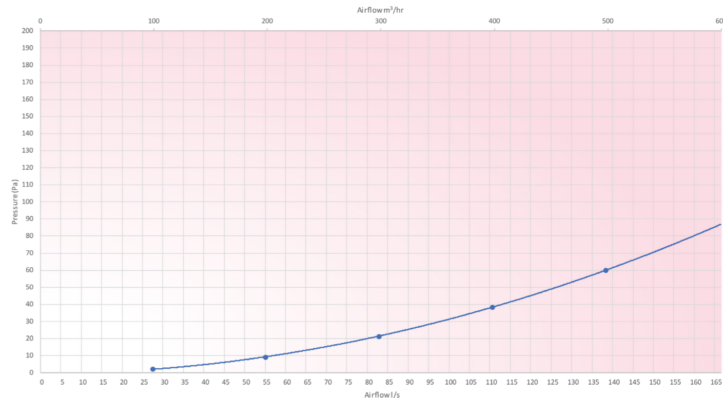
Plastic manifold, 1 x \varnothing 160mm connection, 10 x \varnothing 75mm ports
