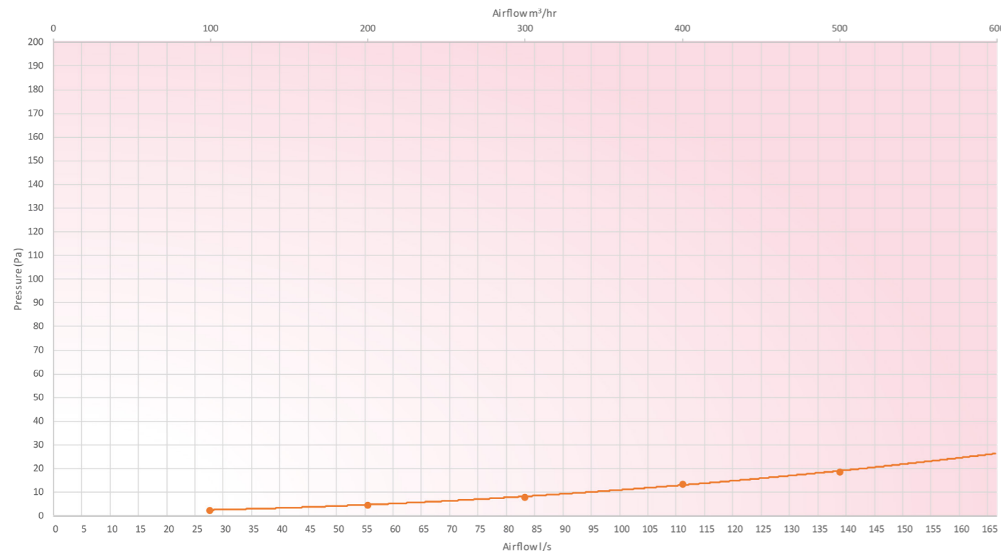
Plastic manifold, 1 x \varnothing 180mm connection, 10 x \varnothing 75mm ports
